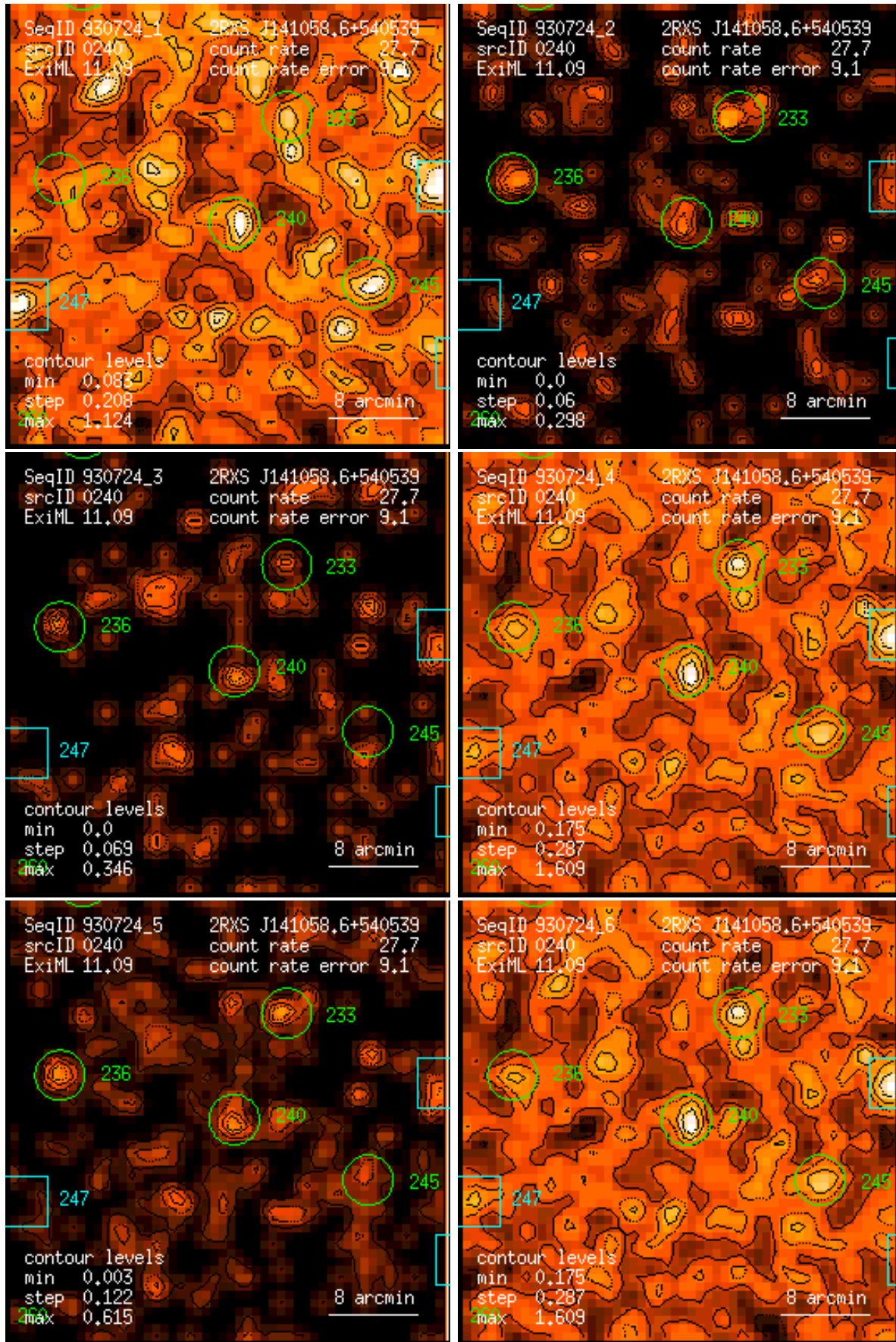
Figure 240: RASS 930724: detection 0240: band rate images, Gaussian filter: (1) PSPC channels 11 – 41, (2) 52 – 90, (3) 91 – 201, (4) 11 – 235, (5) 52 – 201, (6) 11 – 201. Broad band rates in counts/ks. Band rate contour levels in counts/ks/arcmin 2 .
