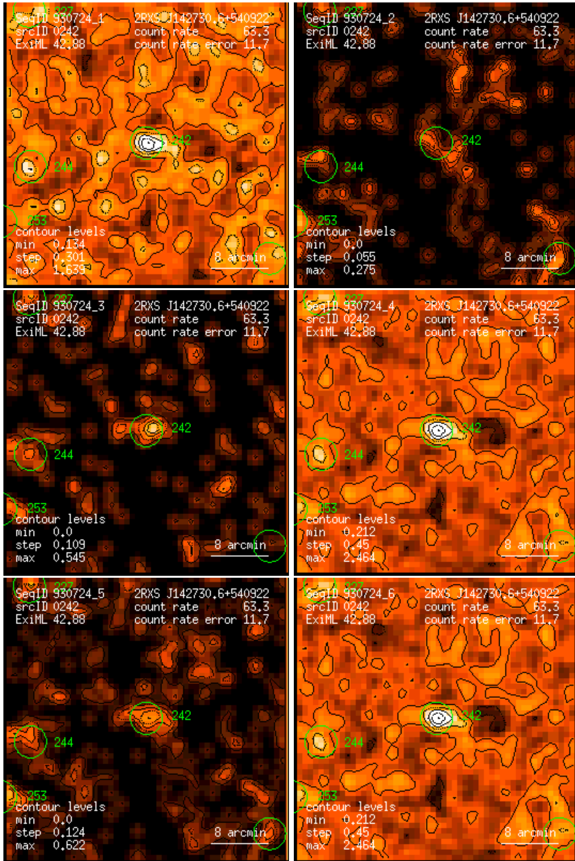
Figure 242: RASS 930724: detection 0242: band rate images, Gaussian filter: (1) PSPC channels 11 – 41, (2) 52 – 90, (3) 91 – 201, (4) 11 – 235, (5) 52 – 201, (6) 11 – 201. Broad band rates in counts/ks. Band rate contour levels in counts/ks/arcmin 2 .
