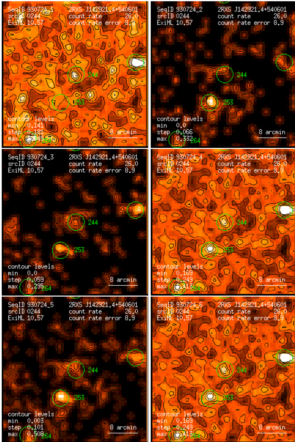
Figure 244: RASS 930724: detection 0244: band rate images, Gaussian filter: (1) PSPC channels 11 – 41, (2) 52 – 90, (3) 91 – 201, (4) 11 – 235, (5) 52 – 201, (6) 11 – 201. Broad band rates in counts/ks. Band rate contour levels in counts/ks/arcmin 2 .
