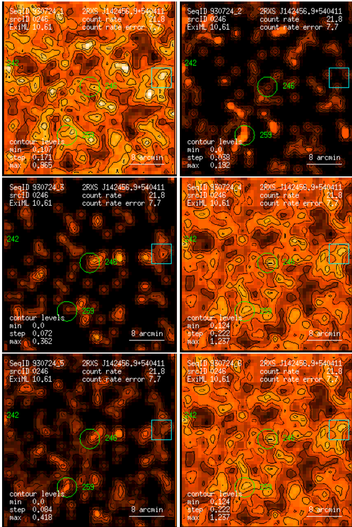
Figure 246: RASS 930724: detection 0246: band rate images, Gaussian filter: (1) PSPC channels 11 – 41, (2) 52 – 90, (3) 91 – 201, (4) 11 – 235, (5) 52 – 201, (6) 11 – 201. Broad band rates in counts/ks. Band rate contour levels in counts/ks/arcmin 2 .
