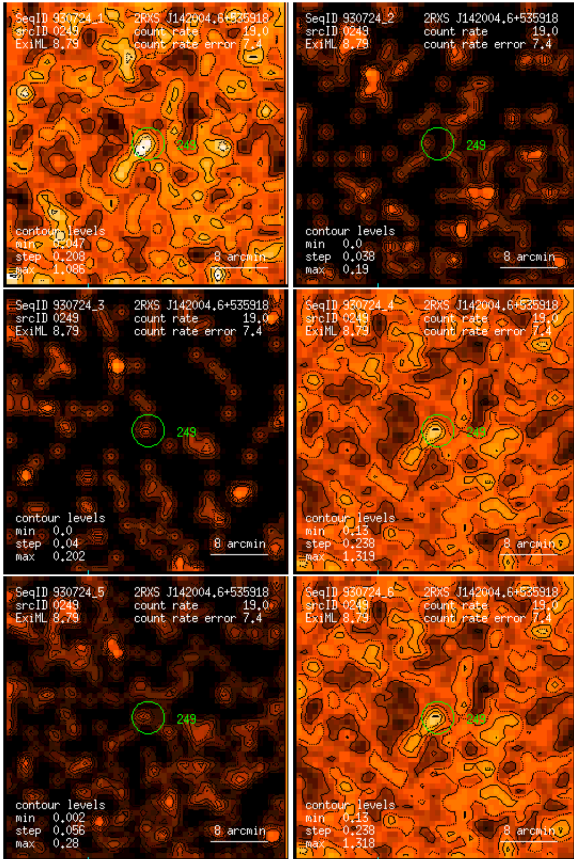
Figure 249: RASS 930724: detection 0249: band rate images, Gaussian filter: (1) PSPC channels 11 – 41, (2) 52 – 90, (3) 91 – 201, (4) 11 – 235, (5) 52 – 201, (6) 11 – 201. Broad band rates in counts/ks. Band rate contour levels in counts/ks/arcmin 2 .
