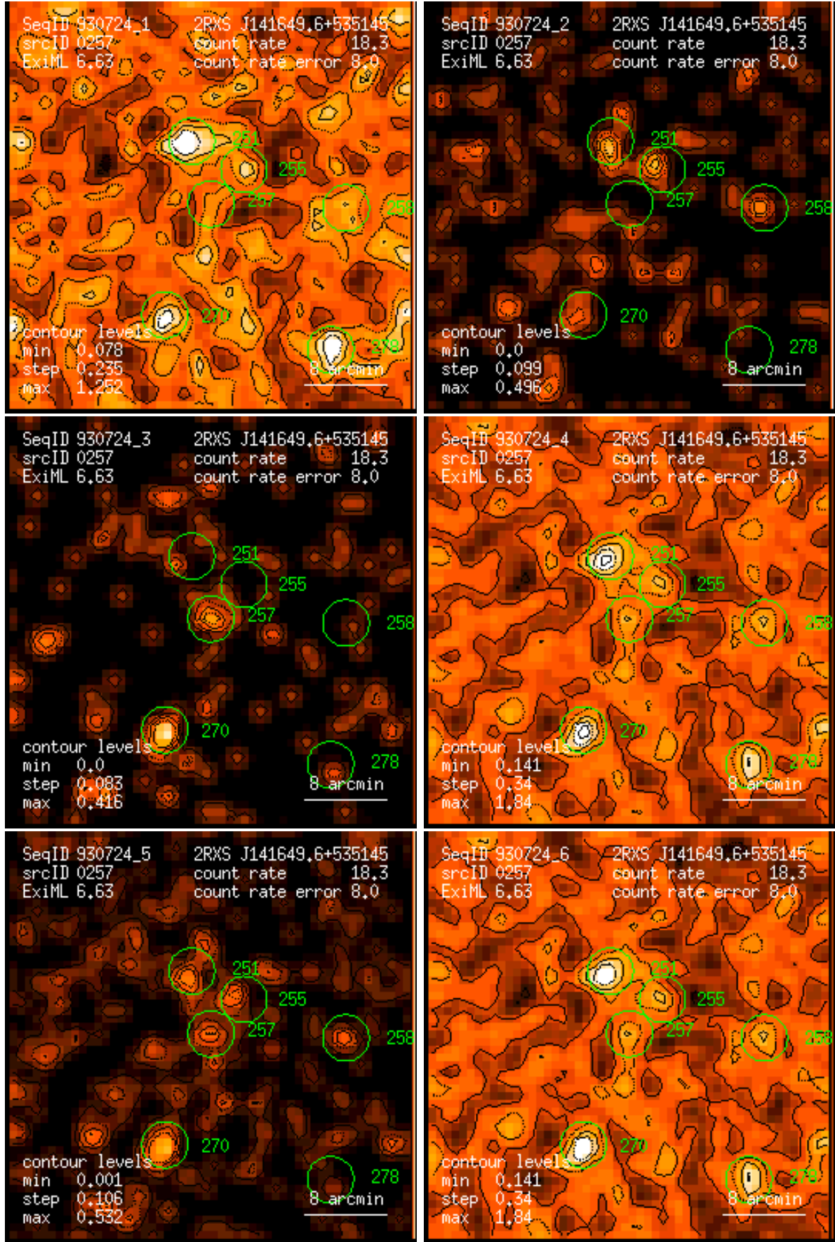
Figure 257: RASS 930724: detection 0257: band rate images, Gaussian filter: (1) PSPC channels 11 – 41, (2) 52 – 90, (3) 91 – 201, (4) 11 – 235, (5) 52 – 201, (6) 11 – 201. Broad band rates in counts/ks. Band rate contour levels in counts/ks/arcmin 2 .
