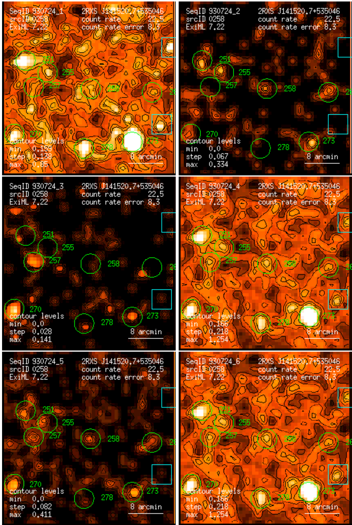
Figure 258: RASS 930724: detection 0258: band rate images, Gaussian filter: (1) PSPC channels 11 – 41, (2) 52 – 90, (3) 91 – 201, (4) 11 – 235, (5) 52 – 201, (6) 11 – 201. Broad band rates in counts/ks. Band rate contour levels in counts/ks/arcmin 2 .
