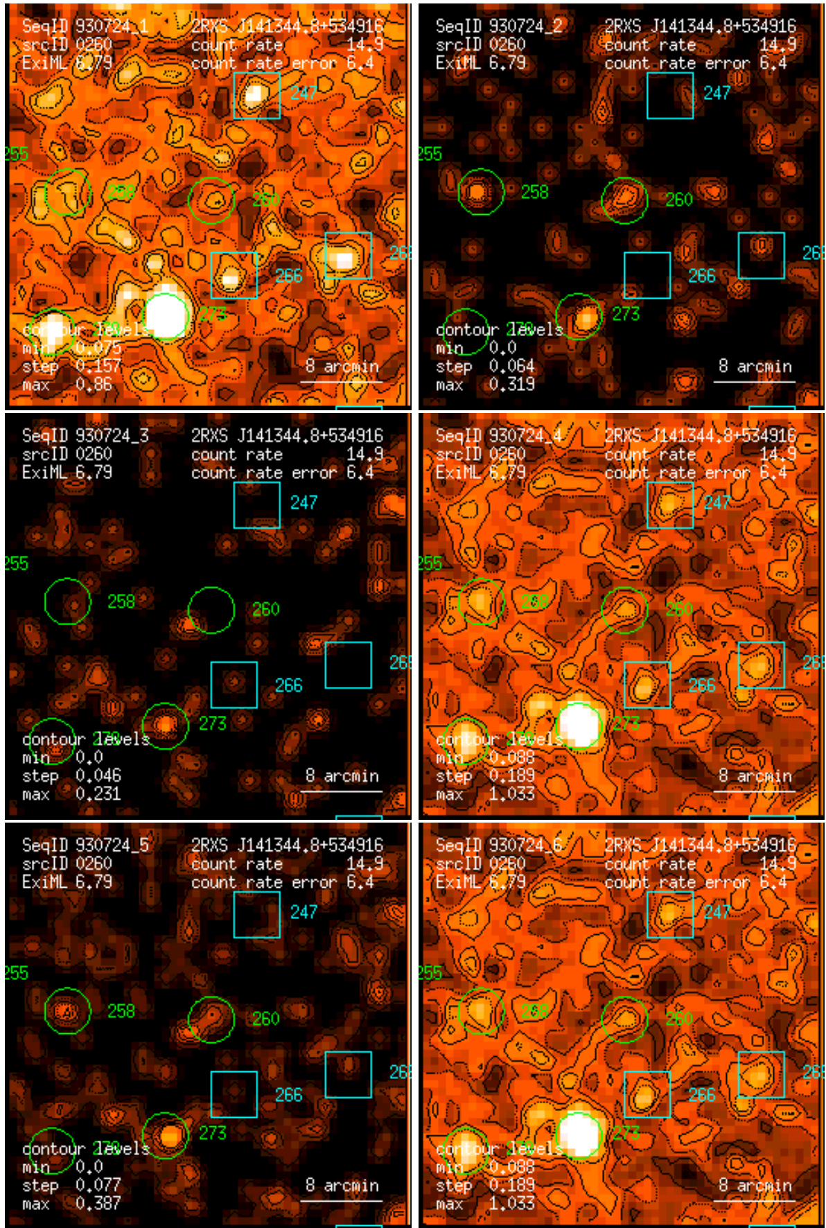
Figure 260: RASS 930724: detection 0260: band rate images, Gaussian filter: (1) PSPC channels 11 – 41, (2) 52 – 90, (3) 91 – 201, (4) 11 – 235, (5) 52 – 201, (6) 11 – 201. Broad band rates in counts/ks. Band rate contour levels in counts/ks/arcmin 2 .
