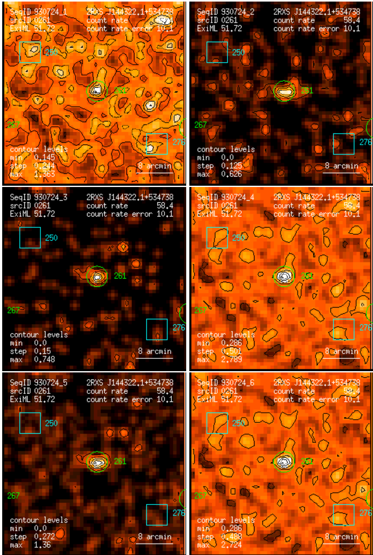
Figure 261: RASS 930724: detection 0261: band rate images, Gaussian filter: (1) PSPC channels 11 – 41, (2) 52 – 90, (3) 91 – 201, (4) 11 – 235, (5) 52 – 201, (6) 11 – 201. Broad band rates in counts/ks. Band rate contour levels in counts/ks/arcmin 2 .
