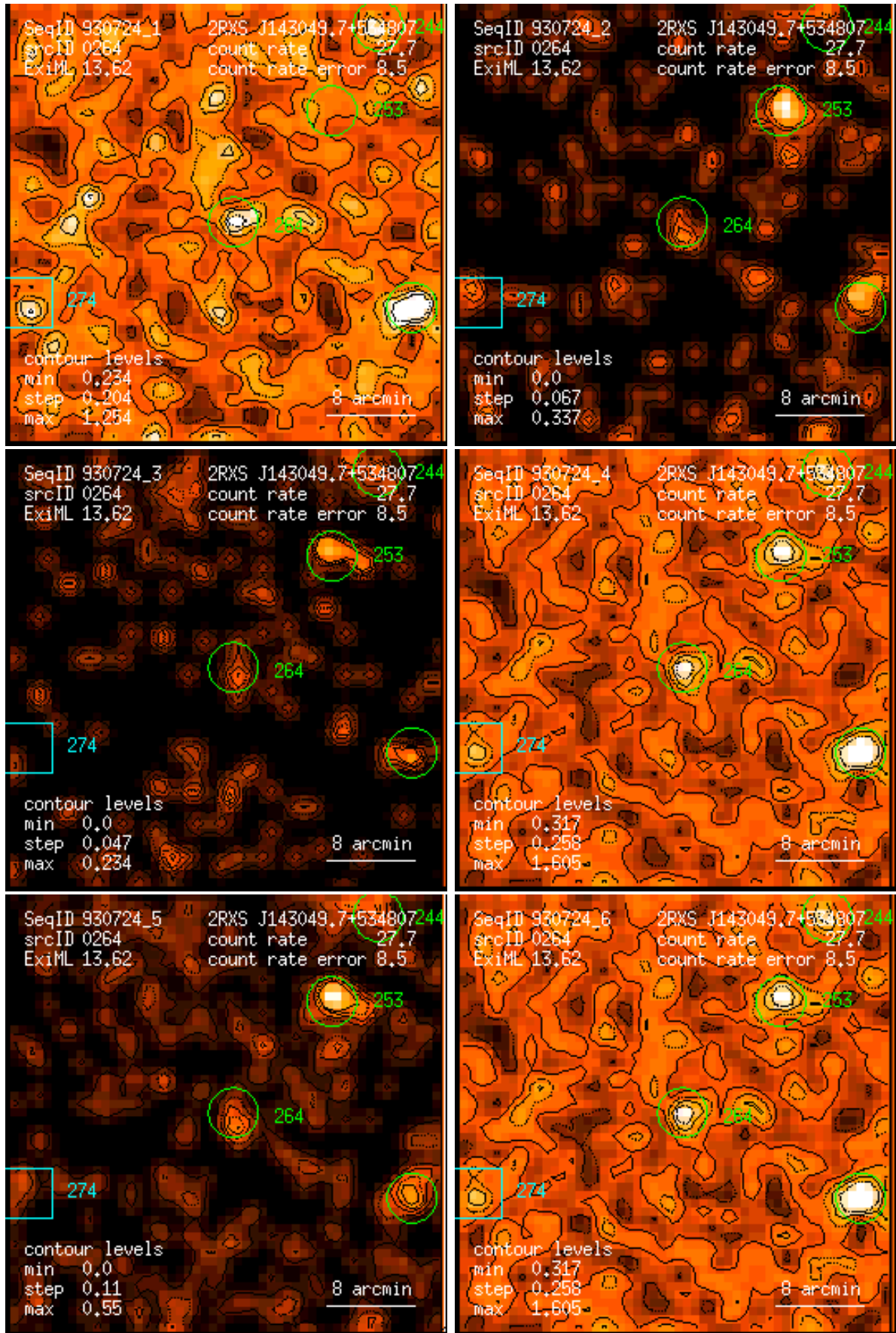
Figure 264: RASS 930724: detection 0264: band rate images, Gaussian filter: (1) PSPC channels 11 – 41, (2) 52 – 90, (3) 91 – 201, (4) 11 – 235, (5) 52 – 201, (6) 11 – 201. Broad band rates in counts/ks. Band rate contour levels in counts/ks/arcmin 2 .
