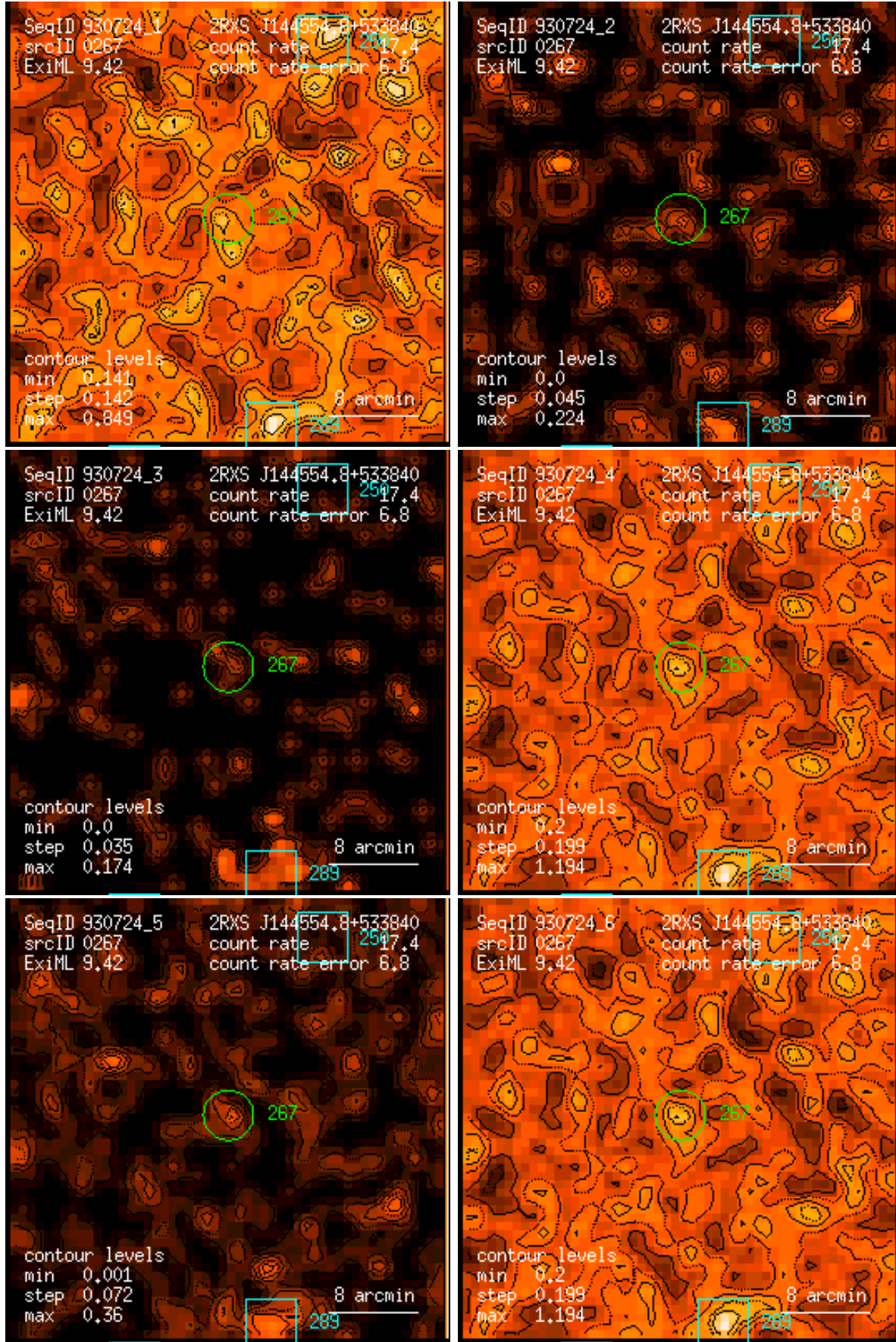
Figure 267: RASS 930724: detection 0267: band rate images, Gaussian filter: (1) PSPC channels 11 – 41, (2) 52 – 90, (3) 91 – 201, (4) 11 – 235, (5) 52 – 201, (6) 11 – 201. Broad band rates in counts/ks. Band rate contour levels in counts/ks/arcmin 2 .
