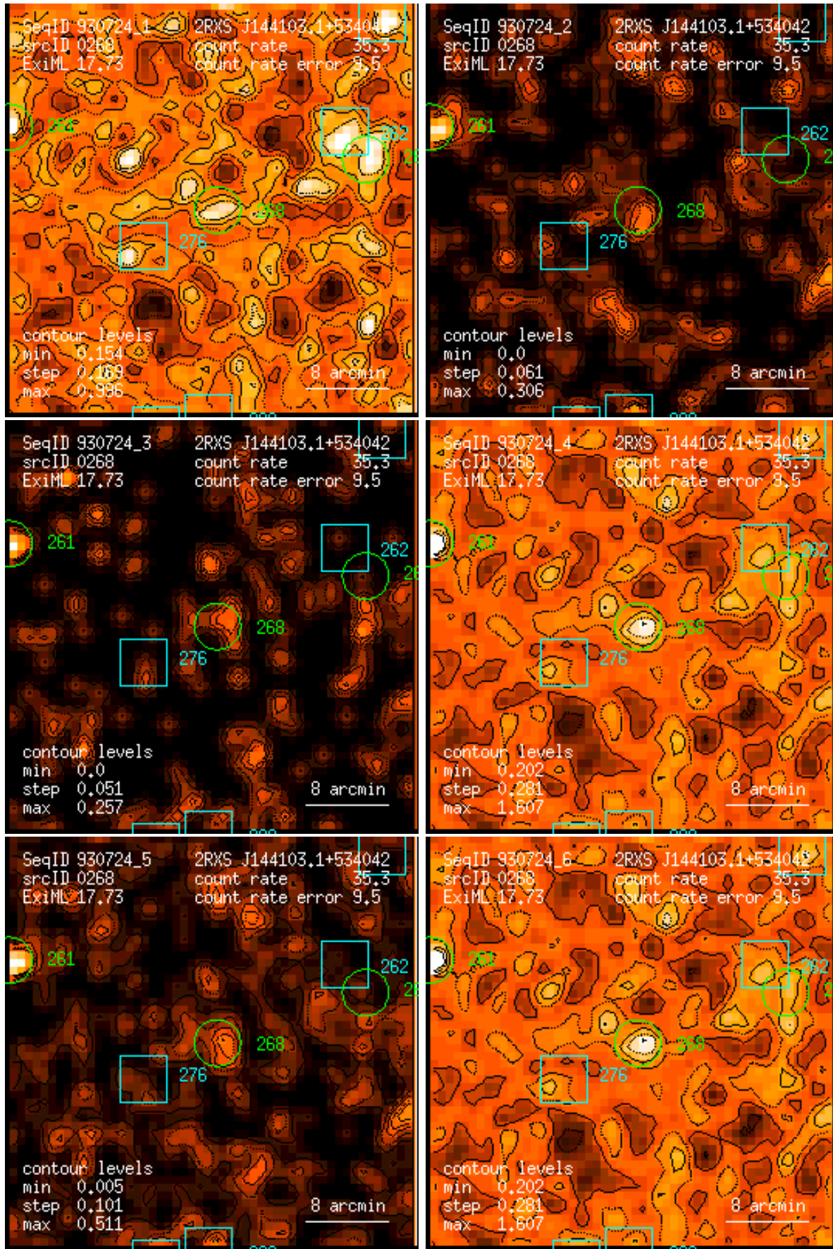
Figure 268: RASS 930724: detection 0268: band rate images, Gaussian filter: (1) PSPC channels 11 – 41, (2) 52 – 90, (3) 91 – 201, (4) 11 – 235, (5) 52 – 201, (6) 11 – 201. Broad band rates in counts/ks. Band rate contour levels in counts/ks/arcmin 2 .
