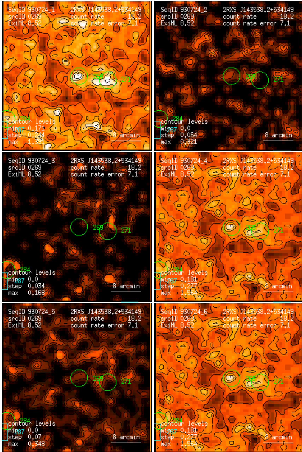
Figure 269: RASS 930724: detection 0269: band rate images, Gaussian filter: (1) PSPC channels 11 – 41, (2) 52 – 90, (3) 91 – 201, (4) 11 – 235, (5) 52 – 201, (6) 11 – 201. Broad band rates in counts/ks. Band rate contour levels in counts/ks/arcmin 2 .
