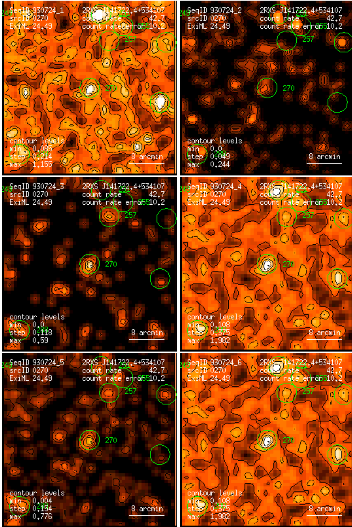
Figure 270: RASS 930724: detection 0270: band rate images, Gaussian filter: (1) PSPC channels 11 – 41, (2) 52 – 90, (3) 91 – 201, (4) 11 – 235, (5) 52 – 201, (6) 11 – 201. Broad band rates in counts/ks. Band rate contour levels in counts/ks/arcmin 2 .
