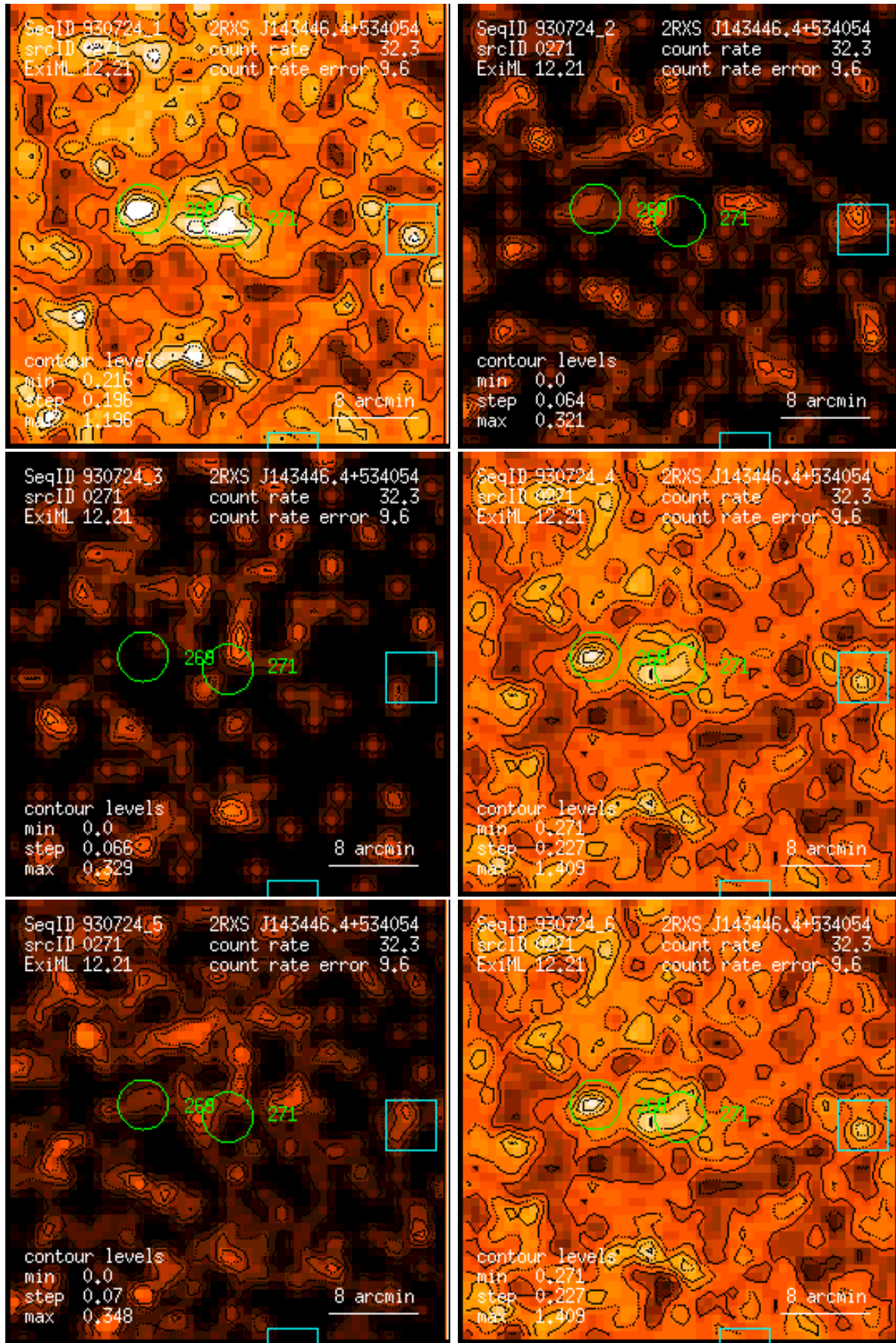
Figure 271: RASS 930724: detection 0271: band rate images, Gaussian filter: (1) PSPC channels 11 – 41, (2) 52 – 90, (3) 91 – 201, (4) 11 – 235, (5) 52 – 201, (6) 11 – 201. Broad band rates in counts/ks. Band rate contour levels in counts/ks/arcmin 2 .
