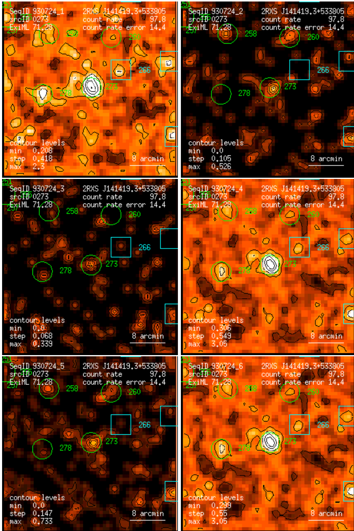
Figure 273: RASS 930724: detection 0273: band rate images, Gaussian filter: (1) PSPC channels 11 – 41, (2) 52 – 90, (3) 91 – 201, (4) 11 – 235, (5) 52 – 201, (6) 11 – 201. Broad band rates in counts/ks. Band rate contour levels in counts/ks/arcmin 2 .
