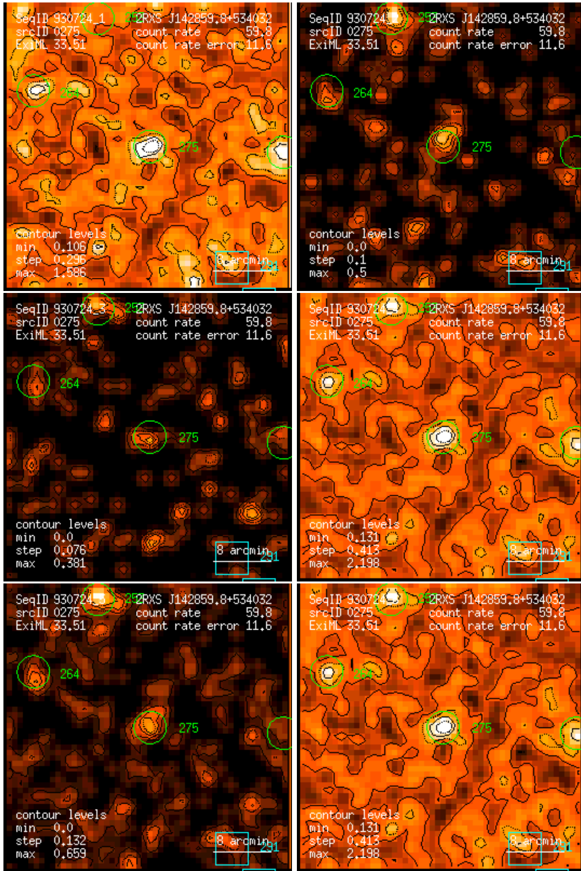
Figure 275: RASS 930724: detection 0275: band rate images, Gaussian filter: (1) PSPC channels 11 – 41, (2) 52 – 90, (3) 91 – 201, (4) 11 – 235, (5) 52 – 201, (6) 11 – 201. Broad band rates in counts/ks. Band rate contour levels in counts/ks/arcmin 2 .
