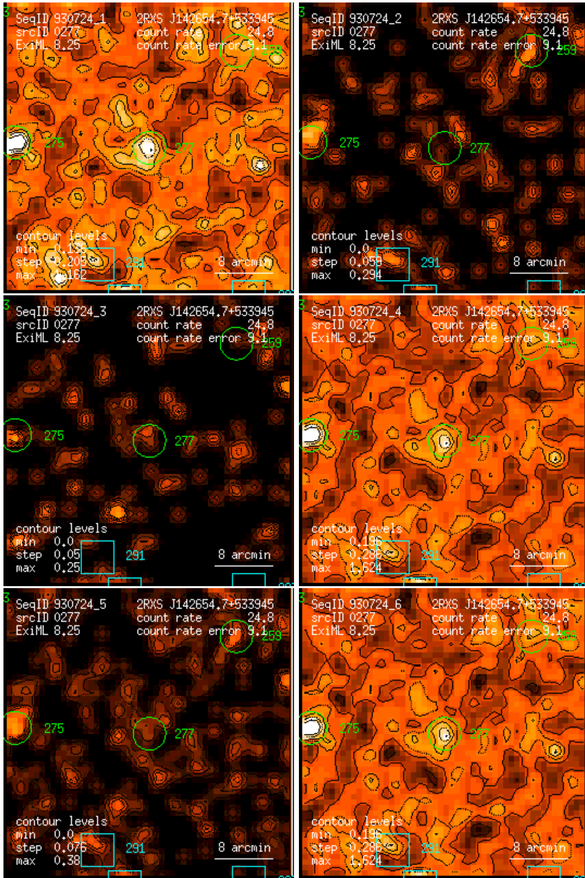
Figure 277: RASS 930724: detection 0277: band rate images, Gaussian filter: (1) PSPC channels 11 – 41, (2) 52 – 90, (3) 91 – 201, (4) 11 – 235, (5) 52 – 201, (6) 11 – 201. Broad band rates in counts/ks. Band rate contour levels in counts/ks/arcmin 2 .
