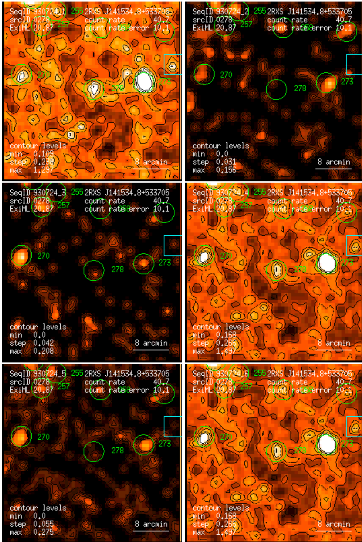
Figure 278: RASS 930724: detection 0278: band rate images, Gaussian filter: (1) PSPC channels 11 – 41, (2) 52 – 90, (3) 91 – 201, (4) 11 – 235, (5) 52 – 201, (6) 11 – 201. Broad band rates in counts/ks. Band rate contour levels in counts/ks/arcmin 2 .
