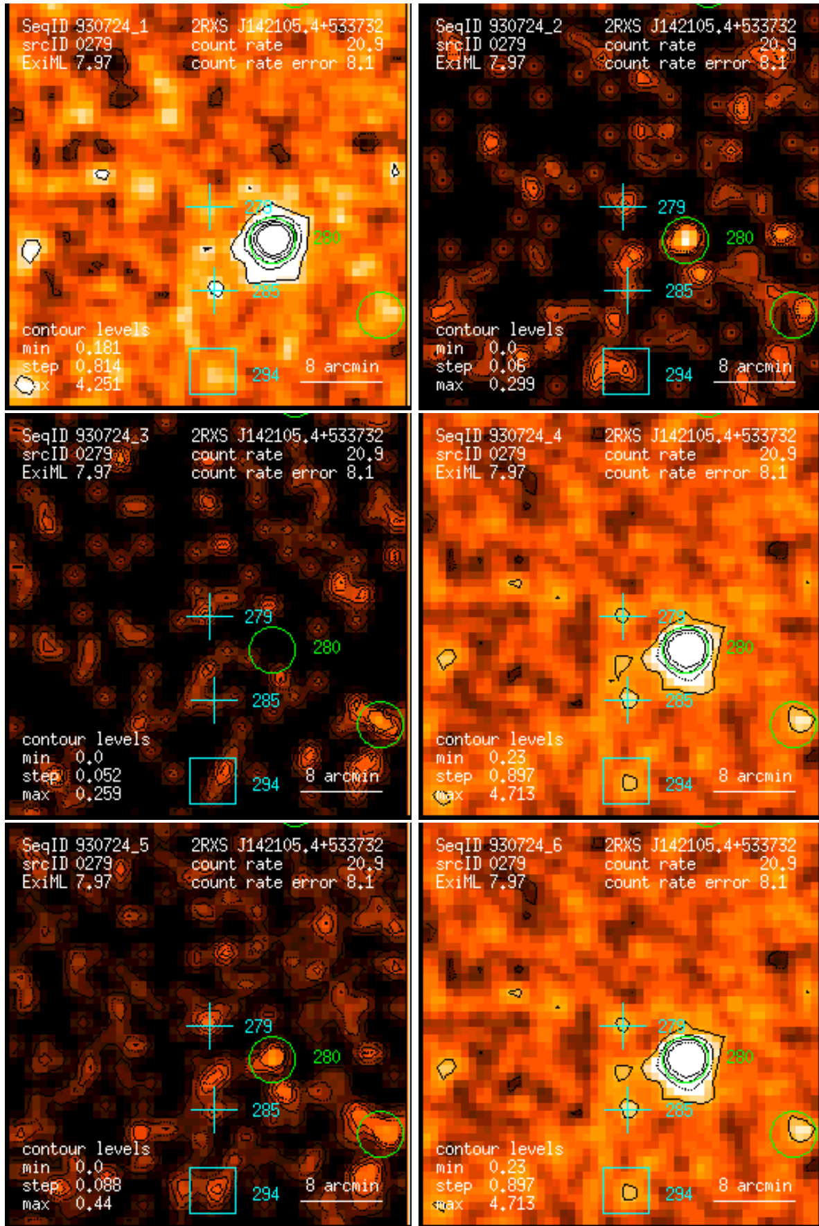
Figure 279: RASS 930724: detection 0279: band rate images, Gaussian filter: (1) PSPC channels 11 – 41, (2) 52 – 90, (3) 91 – 201, (4) 11 – 235, (5) 52 – 201, (6) 11 – 201. Broad band rates in counts/ks. Band rate contour levels in counts/ks/arcmin 2 .
