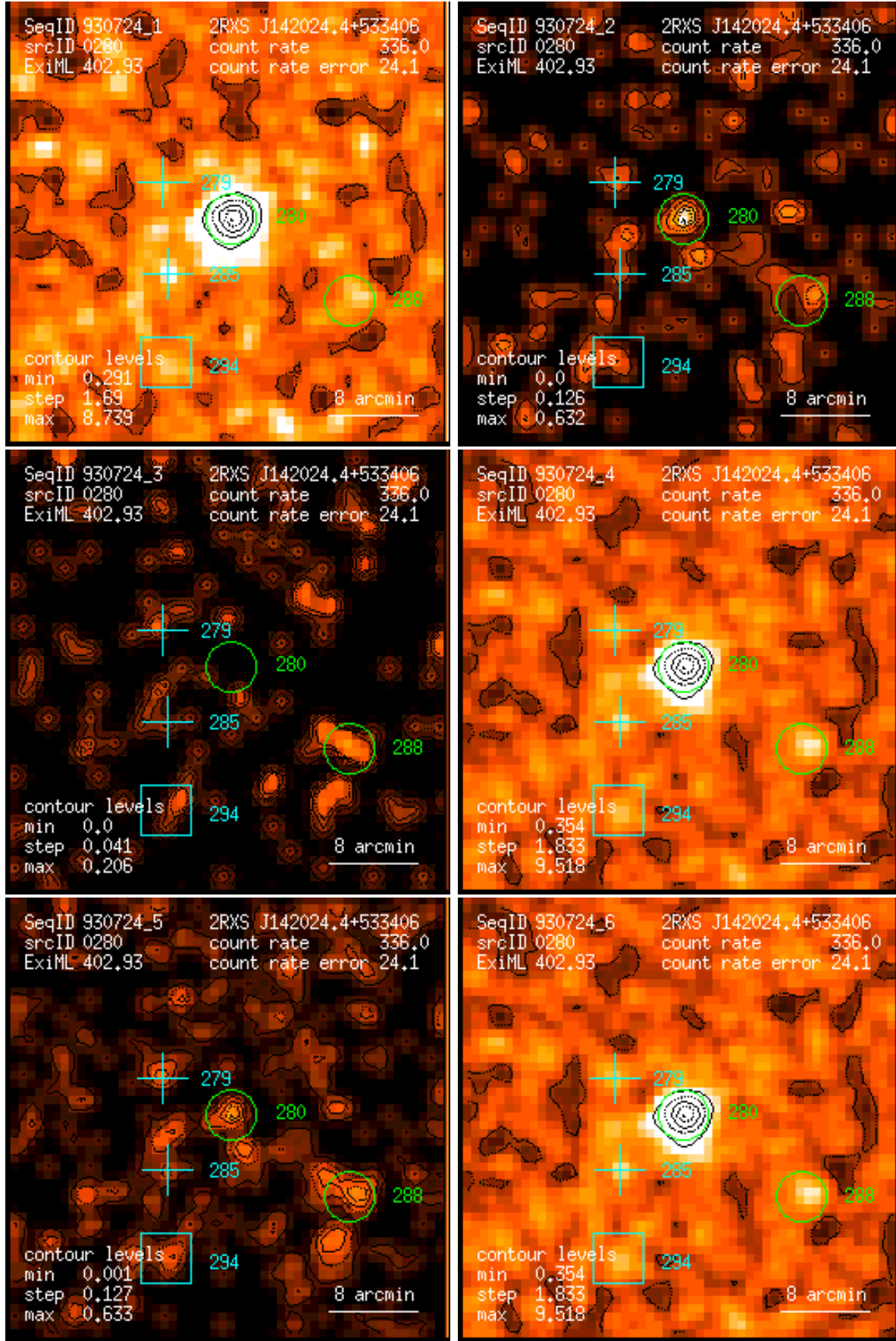
Figure 280: RASS 930724: detection 0280: band rate images, Gaussian filter: (1) PSPC channels 11 – 41, (2) 52 – 90, (3) 91 – 201, (4) 11 – 235, (5) 52 – 201, (6) 11 – 201. Broad band rates in counts/ks. Band rate contour levels in counts/ks/arcmin 2 .
