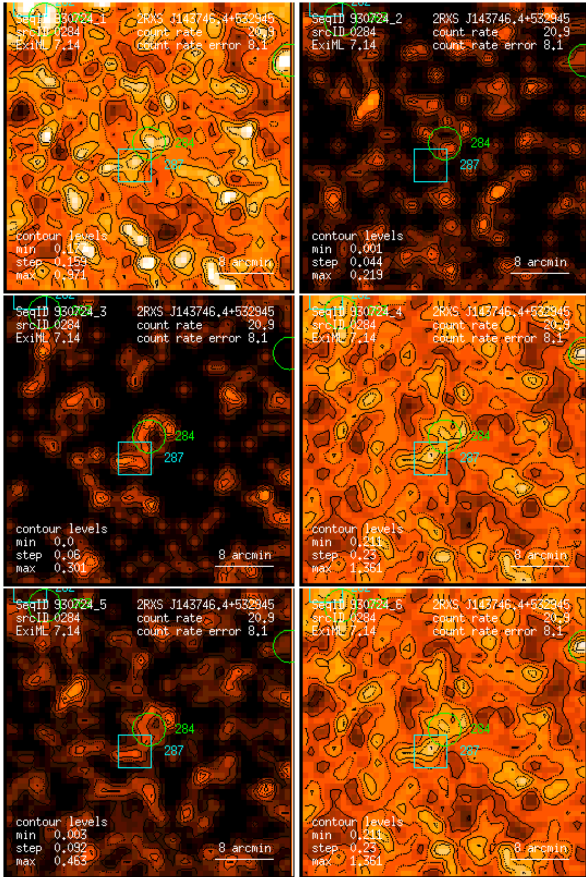
Figure 284: RASS 930724: detection 0284: band rate images, Gaussian filter: (1) PSPC channels 11 – 41, (2) 52 – 90, (3) 91 – 201, (4) 11 – 235, (5) 52 – 201, (6) 11 – 201. Broad band rates in counts/ks. Band rate contour levels in counts/ks/arcmin 2 .
