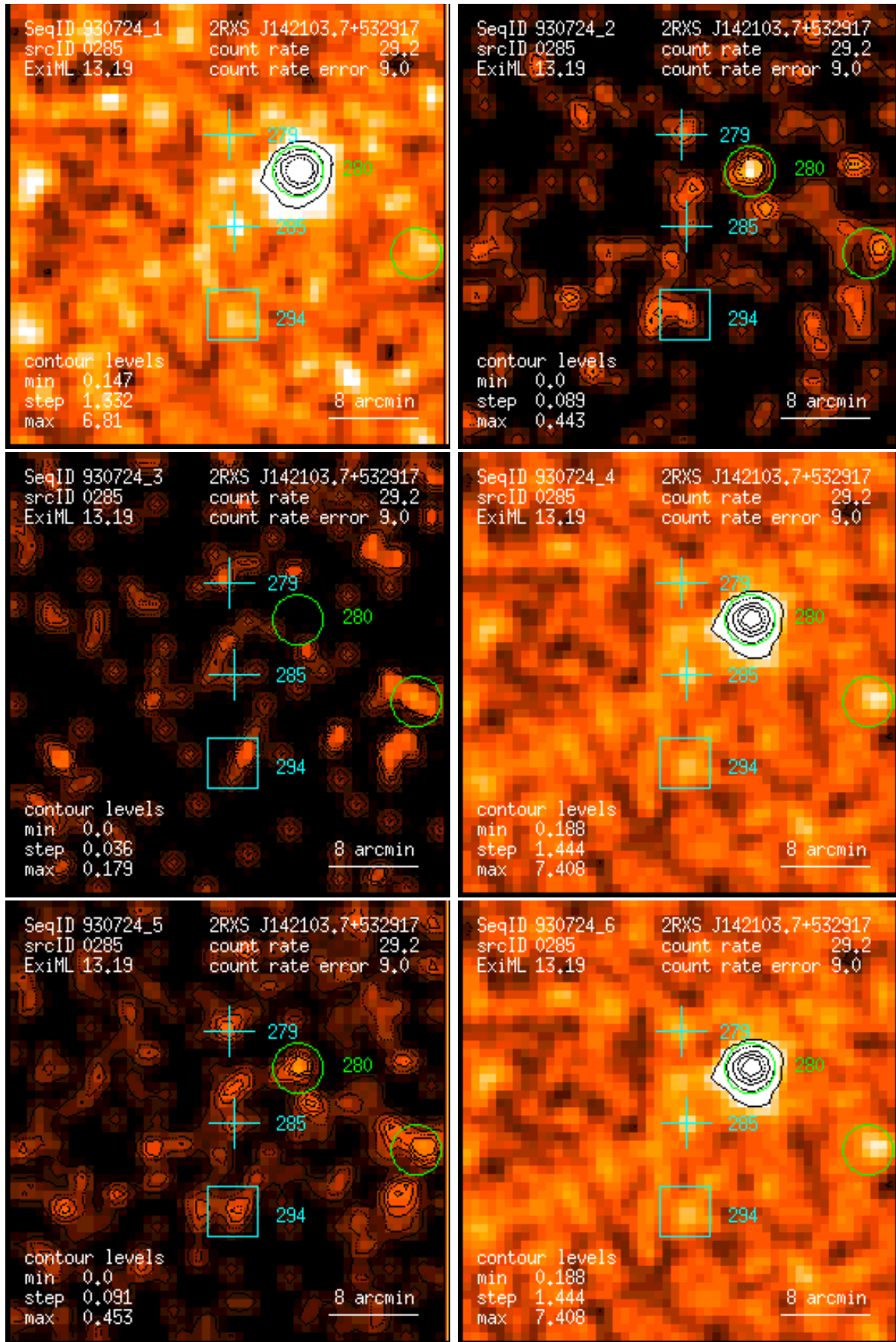
Figure 285: RASS 930724: detection 0285: band rate images, Gaussian filter: (1) PSPC channels 11 – 41, (2) 52 – 90, (3) 91 – 201, (4) 11 – 235, (5) 52 – 201, (6) 11 – 201. Broad band rates in counts/ks. Band rate contour levels in counts/ks/arcmin 2 .
