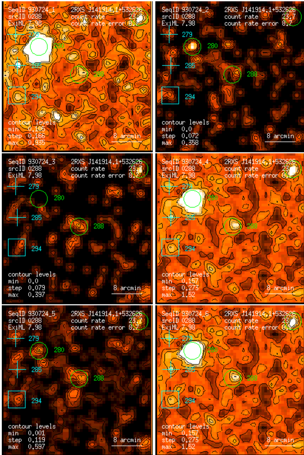
Figure 288: RASS 930724: detection 0288: band rate images, Gaussian filter: (1) PSPC channels 11 – 41, (2) 52 – 90, (3) 91 – 201, (4) 11 – 235, (5) 52 – 201, (6) 11 – 201. Broad band rates in counts/ks. Band rate contour levels in counts/ks/arcmin 2 .
