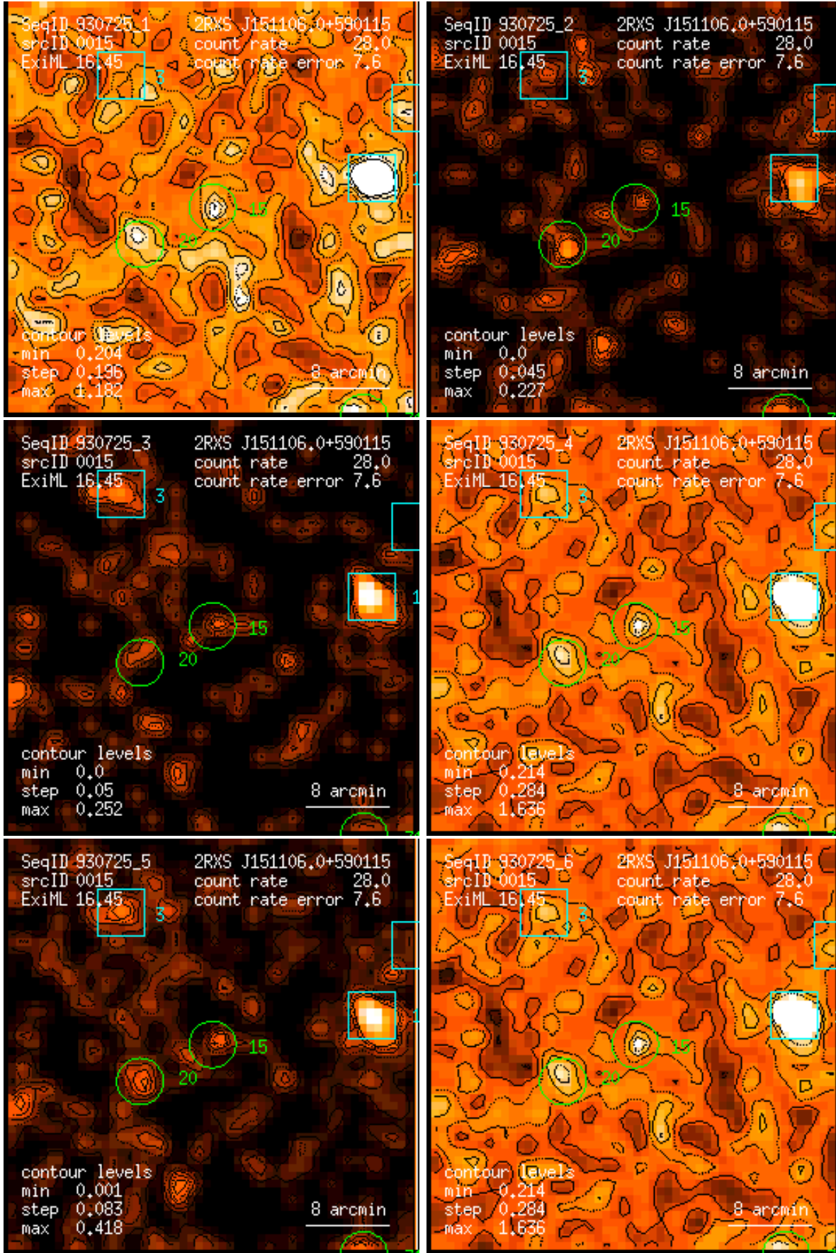
Figure 15: RASS 930725: detection 0015: band rate images, Gaussian filter: (1) PSPC channels 11 – 41, (2) 52 – 90, (3) 91 – 201, (4) 11 – 235, (5) 52 – 201, (6) 11 – 201. Broad band rates in counts/ks. Band rate contour levels in counts/ks/arcmin 2 .
