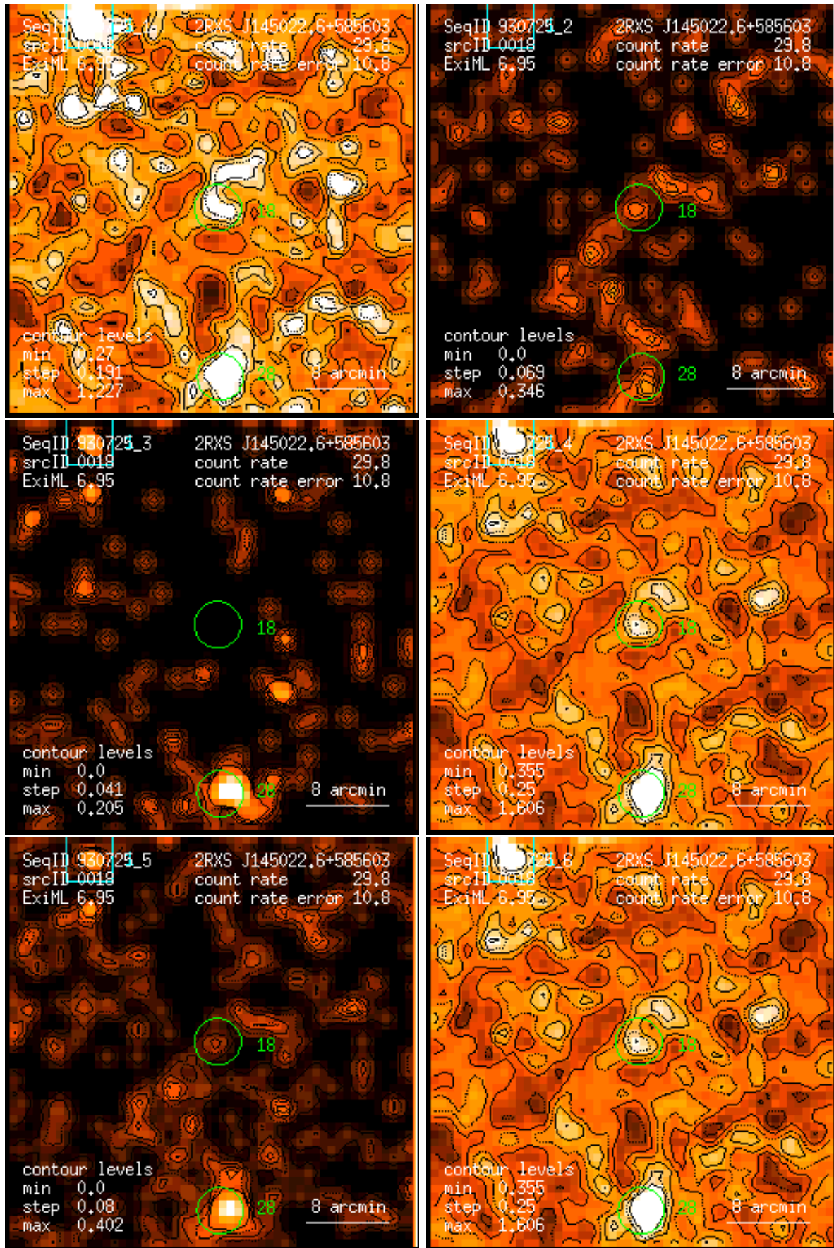
Figure 18: RASS 930725: detection 0018: band rate images, Gaussian filter: (1) PSPC channels 11 – 41, (2) 52 – 90, (3) 91 – 201, (4) 11 – 235, (5) 52 – 201, (6) 11 – 201. Broad band rates in counts/ks. Band rate contour levels in counts/ks/arcmin 2 .
