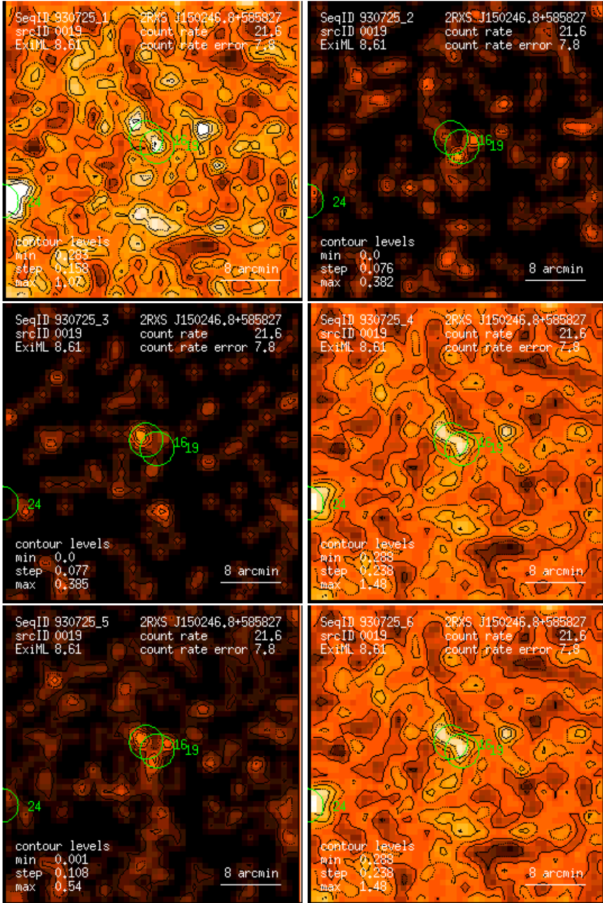
Figure 19: RASS 930725: detection 0019: band rate images, Gaussian filter: (1) PSPC channels 11 – 41, (2) 52 – 90, (3) 91 – 201, (4) 11 – 235, (5) 52 – 201, (6) 11 – 201. Broad band rates in counts/ks. Band rate contour levels in counts/ks/arcmin 2 .
