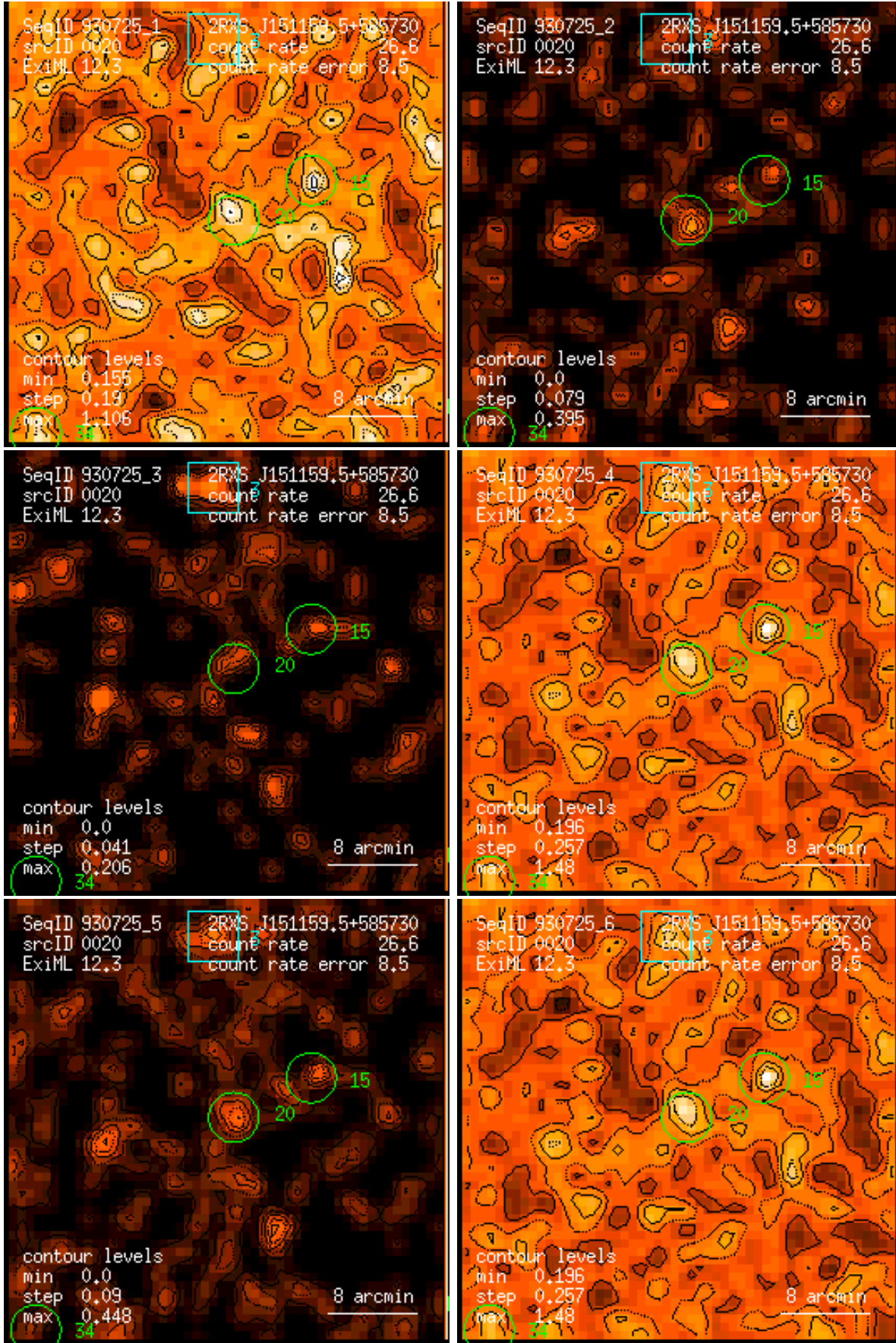
Figure 20: RASS 930725: detection 0020: band rate images, Gaussian filter: (1) PSPC channels 11 – 41, (2) 52 – 90, (3) 91 – 201, (4) 11 – 235, (5) 52 – 201, (6) 11 – 201. Broad band rates in counts/ks. Band rate contour levels in counts/ks/arcmin 2 .
