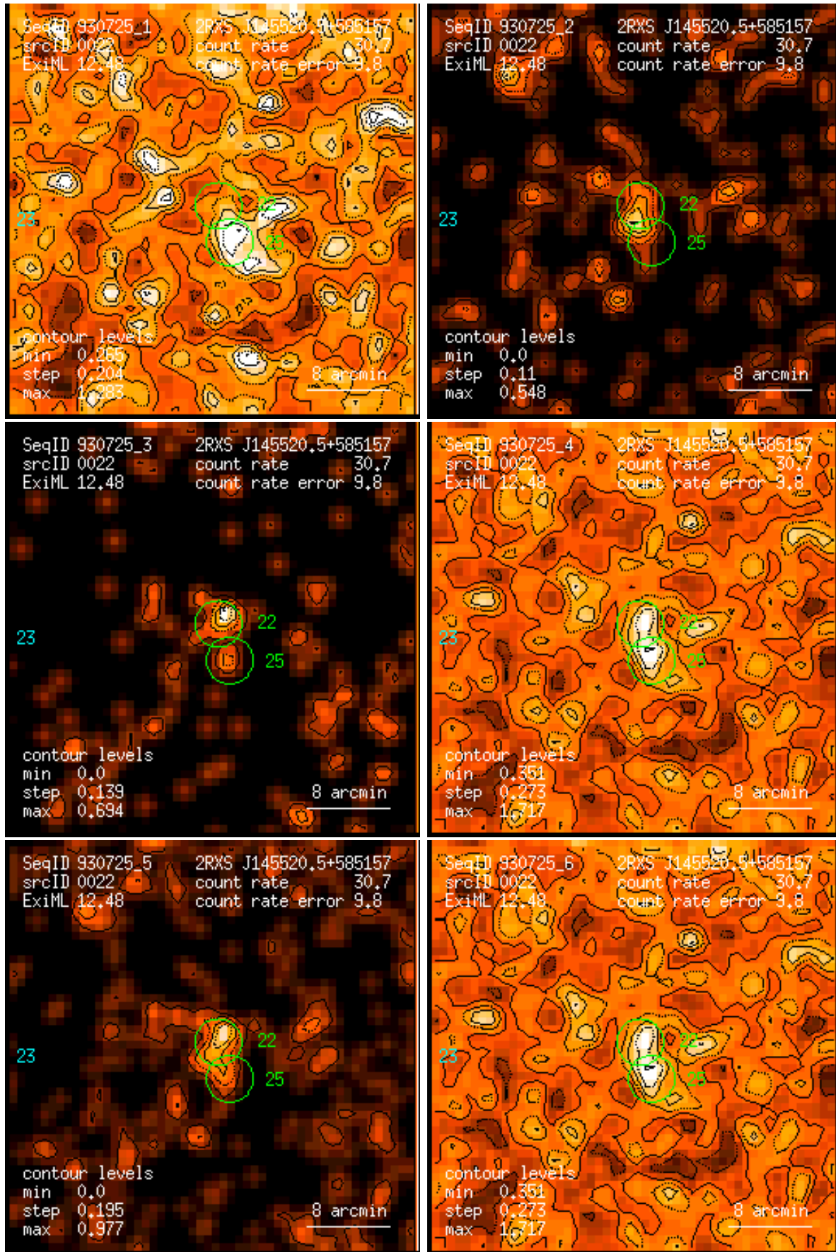
Figure 22: RASS 930725: detection 0022: band rate images, Gaussian filter: (1) PSPC channels 11 – 41, (2) 52 – 90, (3) 91 – 201, (4) 11 – 235, (5) 52 – 201, (6) 11 – 201. Broad band rates in counts/ks. Band rate contour levels in counts/ks/arcmin 2 .
