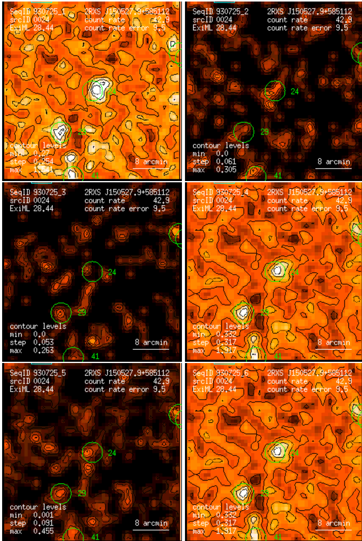
Figure 24: RASS 930725: detection 0024: band rate images, Gaussian filter: (1) PSPC channels 11 – 41, (2) 52 – 90, (3) 91 – 201, (4) 11 – 235, (5) 52 – 201, (6) 11 – 201. Broad band rates in counts/ks. Band rate contour levels in counts/ks/arcmin 2 .
