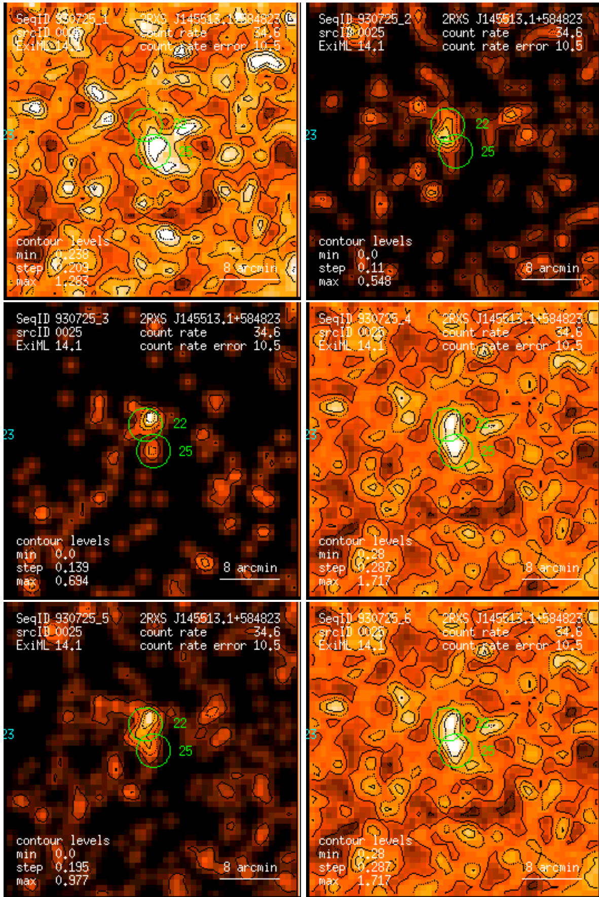
Figure 25: RASS 930725: detection 0025: band rate images, Gaussian filter: (1) PSPC channels 11 – 41, (2) 52 – 90, (3) 91 – 201, (4) 11 – 235, (5) 52 – 201, (6) 11 – 201. Broad band rates in counts/ks. Band rate contour levels in counts/ks/arcmin 2 .
