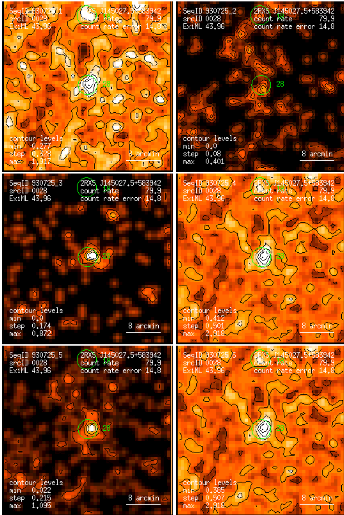
Figure 28: RASS 930725: detection 0028: band rate images, Gaussian filter: (1) PSPC channels 11 – 41, (2) 52 – 90, (3) 91 – 201, (4) 11 – 235, (5) 52 – 201, (6) 11 – 201. Broad band rates in counts/ks. Band rate contour levels in counts/ks/arcmin 2 .
