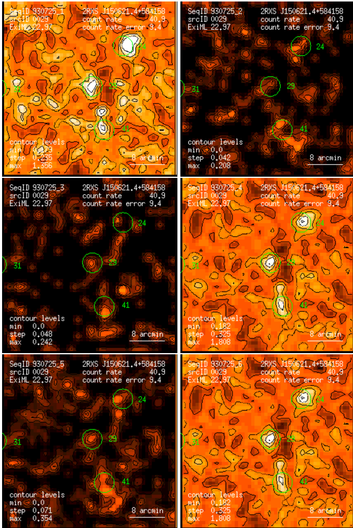
Figure 29: RASS 930725: detection 0029: band rate images, Gaussian filter: (1) PSPC channels 11 – 41, (2) 52 – 90, (3) 91 – 201, (4) 11 – 235, (5) 52 – 201, (6) 11 – 201. Broad band rates in counts/ks. Band rate contour levels in counts/ks/arcmin 2 .
