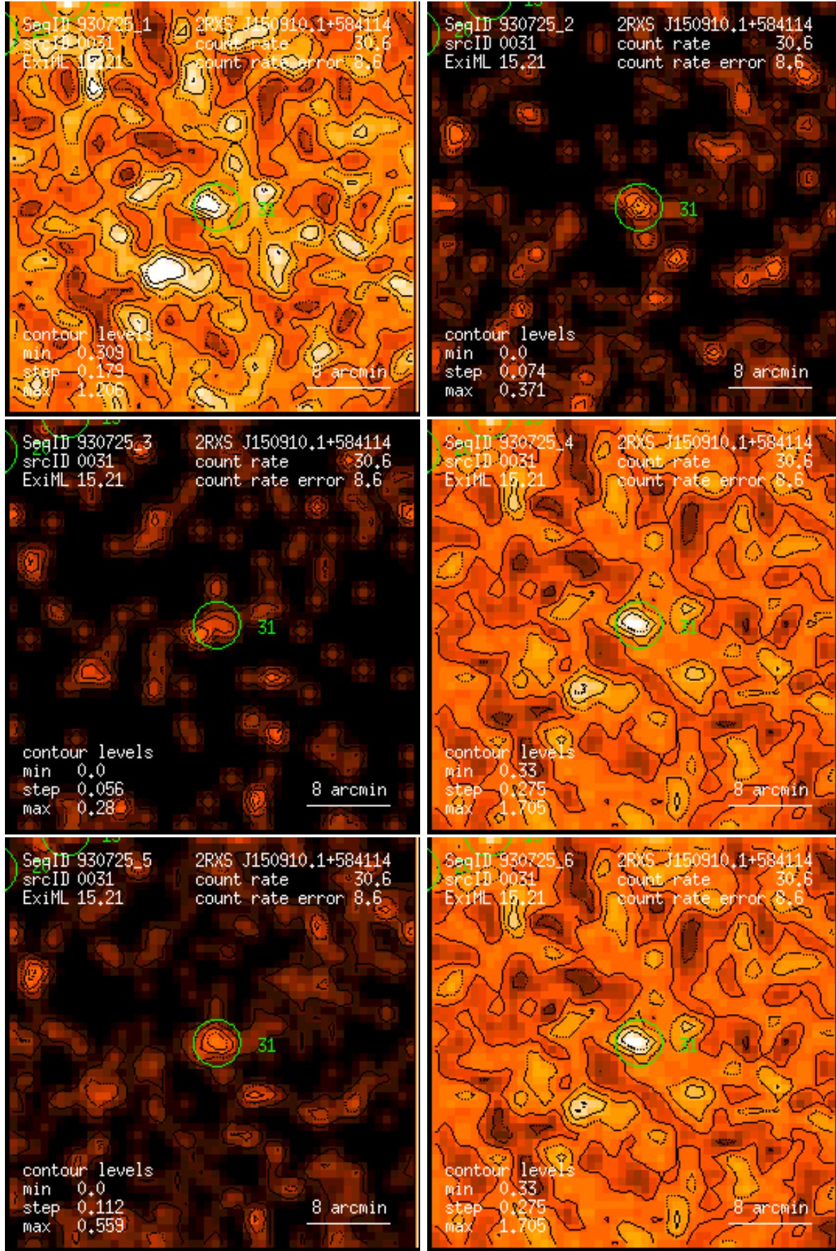
Figure 31: RASS 930725: detection 0031: band rate images, Gaussian filter: (1) PSPC channels 11 – 41, (2) 52 – 90, (3) 91 – 201, (4) 11 – 235, (5) 52 – 201, (6) 11 – 201. Broad band rates in counts/ks. Band rate contour levels in counts/ks/arcmin 2 .
