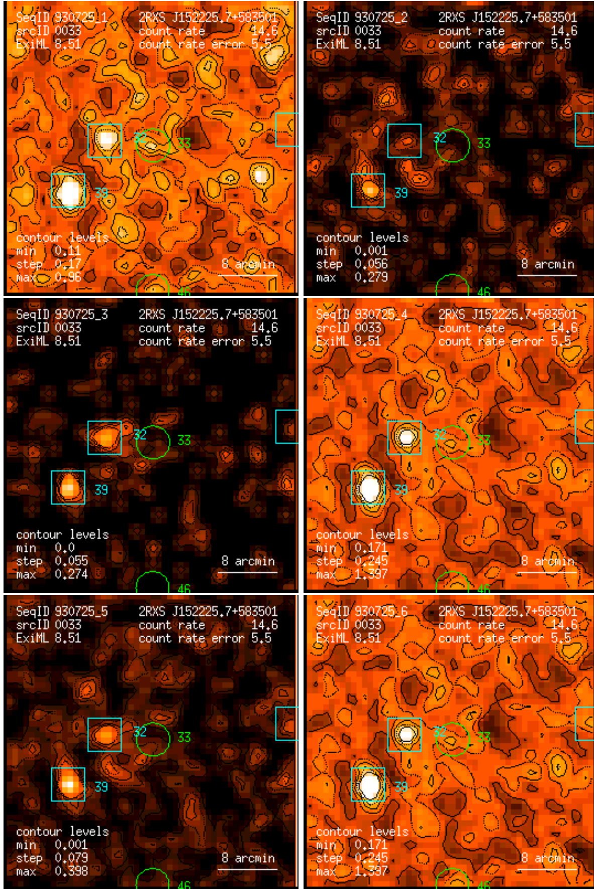
Figure 33: RASS 930725: detection 0033: band rate images, Gaussian filter: (1) PSPC channels 11 – 41, (2) 52 – 90, (3) 91 – 201, (4) 11 – 235, (5) 52 – 201, (6) 11 – 201. Broad band rates in counts/ks. Band rate contour levels in counts/ks/arcmin 2 .
