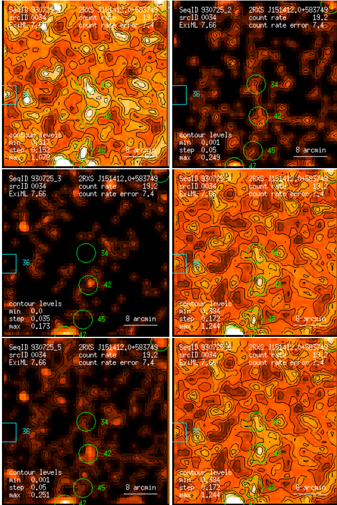
Figure 34: RASS 930725: detection 0034: band rate images, Gaussian filter: (1) PSPC channels 11 – 41, (2) 52 – 90, (3) 91 – 201, (4) 11 – 235, (5) 52 – 201, (6) 11 – 201. Broad band rates in counts/ks. Band rate contour levels in counts/ks/arcmin 2 .
