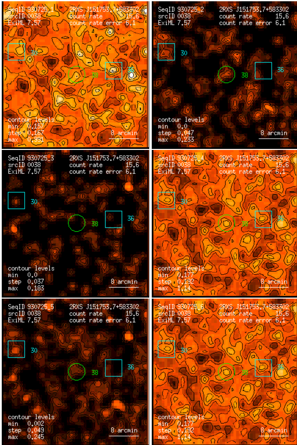
Figure 38: RASS 930725: detection 0038: band rate images, Gaussian filter: (1) PSPC channels 11 – 41, (2) 52 – 90, (3) 91 – 201, (4) 11 – 235, (5) 52 – 201, (6) 11 – 201. Broad band rates in counts/ks. Band rate contour levels in counts/ks/arcmin 2 .
