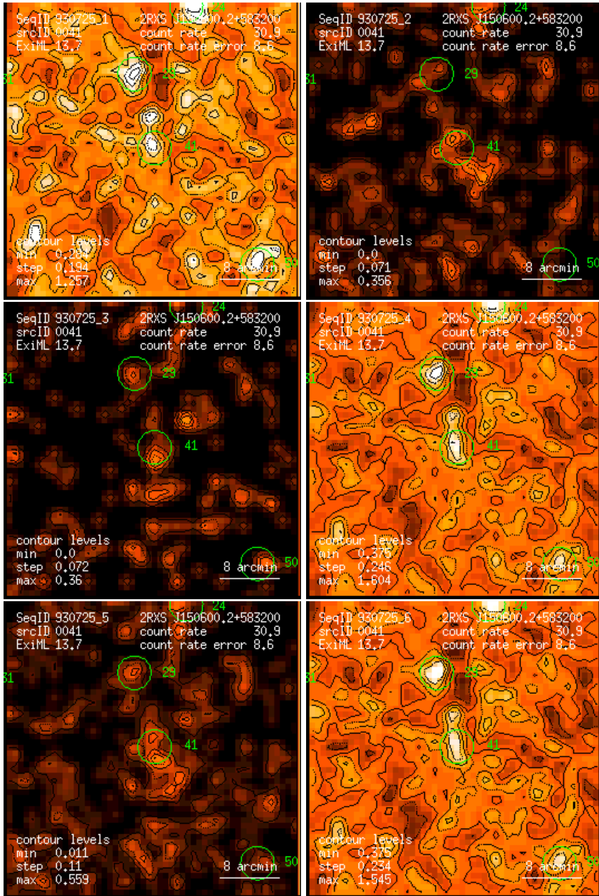
Figure 41: RASS 930725: detection 0041: band rate images, Gaussian filter: (1) PSPC channels 11 – 41, (2) 52 – 90, (3) 91 – 201, (4) 11 – 235, (5) 52 – 201, (6) 11 – 201. Broad band rates in counts/ks. Band rate contour levels in counts/ks/arcmin 2 .
