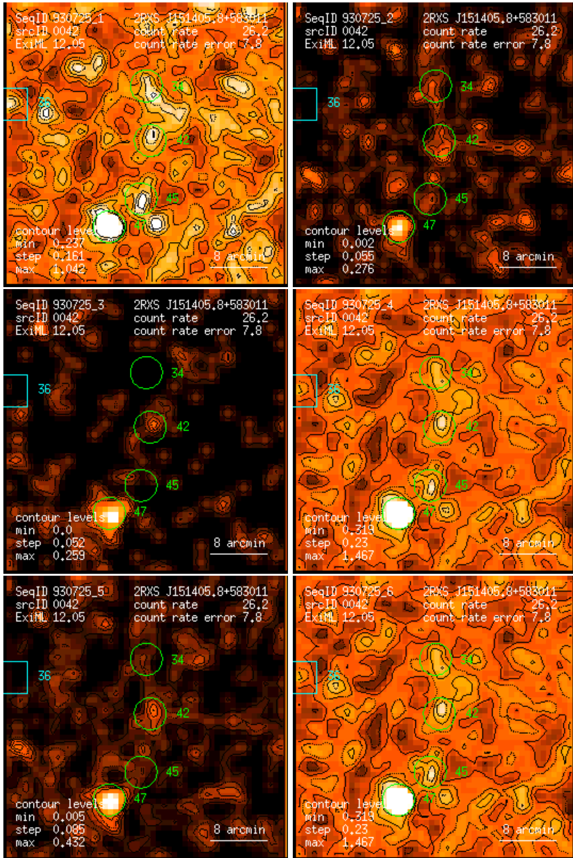
Figure 42: RASS 930725: detection 0042: band rate images, Gaussian filter: (1) PSPC channels 11 – 41, (2) 52 – 90, (3) 91 – 201, (4) 11 – 235, (5) 52 – 201, (6) 11 – 201. Broad band rates in counts/ks. Band rate contour levels in counts/ks/arcmin 2 .
