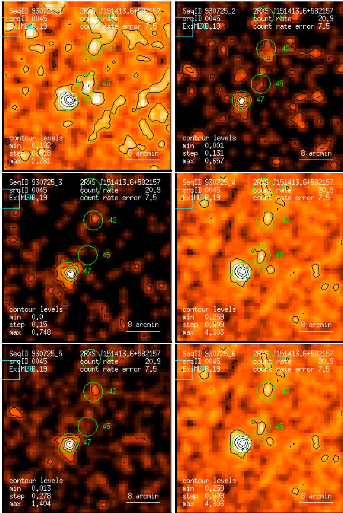
Figure 45: RASS 930725: detection 0045: band rate images, Gaussian filter: (1) PSPC channels 11 – 41, (2) 52 – 90, (3) 91 – 201, (4) 11 – 235, (5) 52 – 201, (6) 11 – 201. Broad band rates in counts/ks. Band rate contour levels in counts/ks/arcmin 2 .
