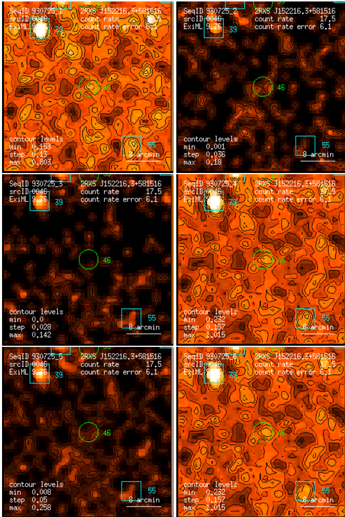
Figure 46: RASS 930725: detection 0046: band rate images, Gaussian filter: (1) PSPC channels 11 – 41, (2) 52 – 90, (3) 91 – 201, (4) 11 – 235, (5) 52 – 201, (6) 11 – 201. Broad band rates in counts/ks. Band rate contour levels in counts/ks/arcmin 2 .
