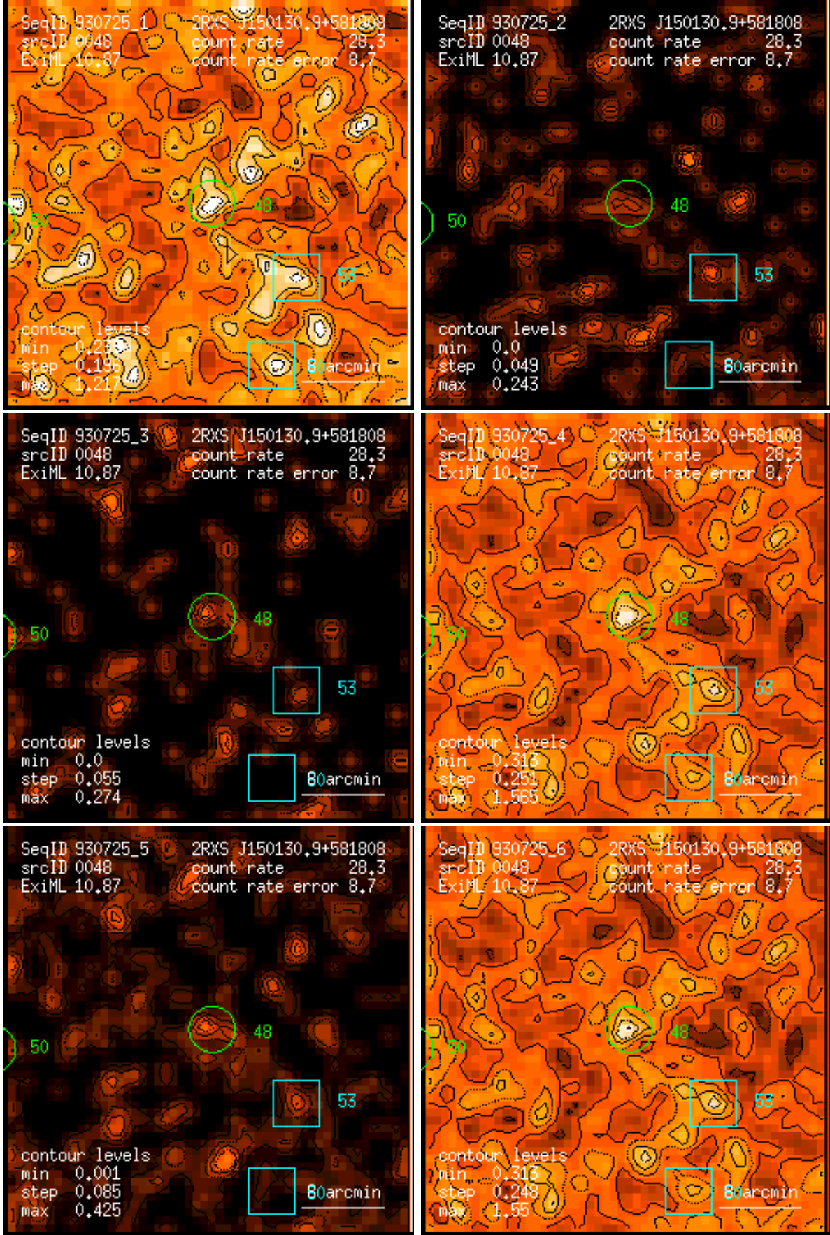
Figure 48: RASS 930725: detection 0048: band rate images, Gaussian filter: (1) PSPC channels 11 – 41, (2) 52 – 90, (3) 91 – 201, (4) 11 – 235, (5) 52 – 201, (6) 11 – 201. Broad band rates in counts/ks. Band rate contour levels in counts/ks/arcmin 2 .
