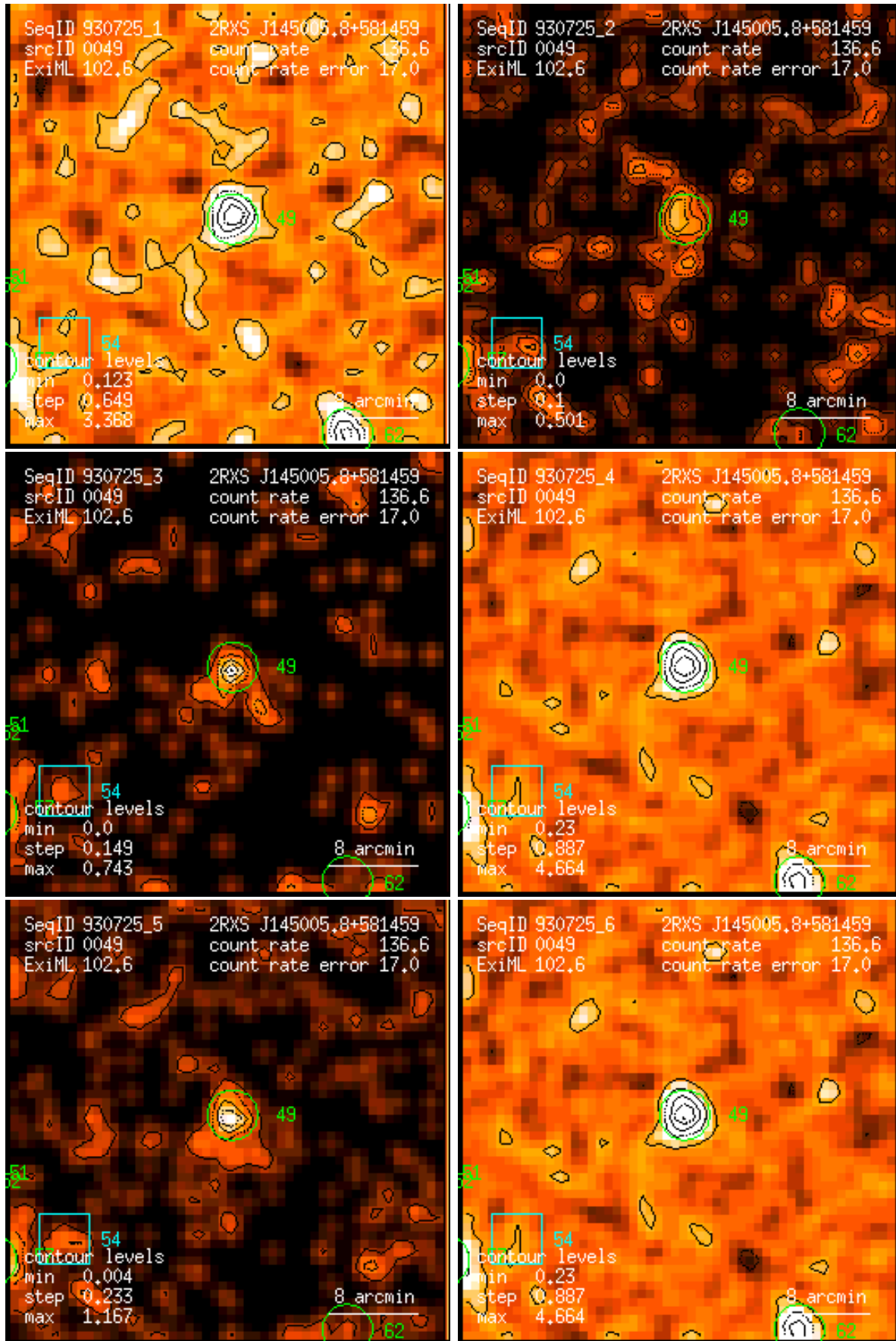
Figure 49: RASS 930725: detection 0049: band rate images, Gaussian filter: (1) PSPC channels 11 – 41, (2) 52 – 90, (3) 91 – 201, (4) 11 – 235, (5) 52 – 201, (6) 11 – 201. Broad band rates in counts/ks. Band rate contour levels in counts/ks/arcmin 2 .
