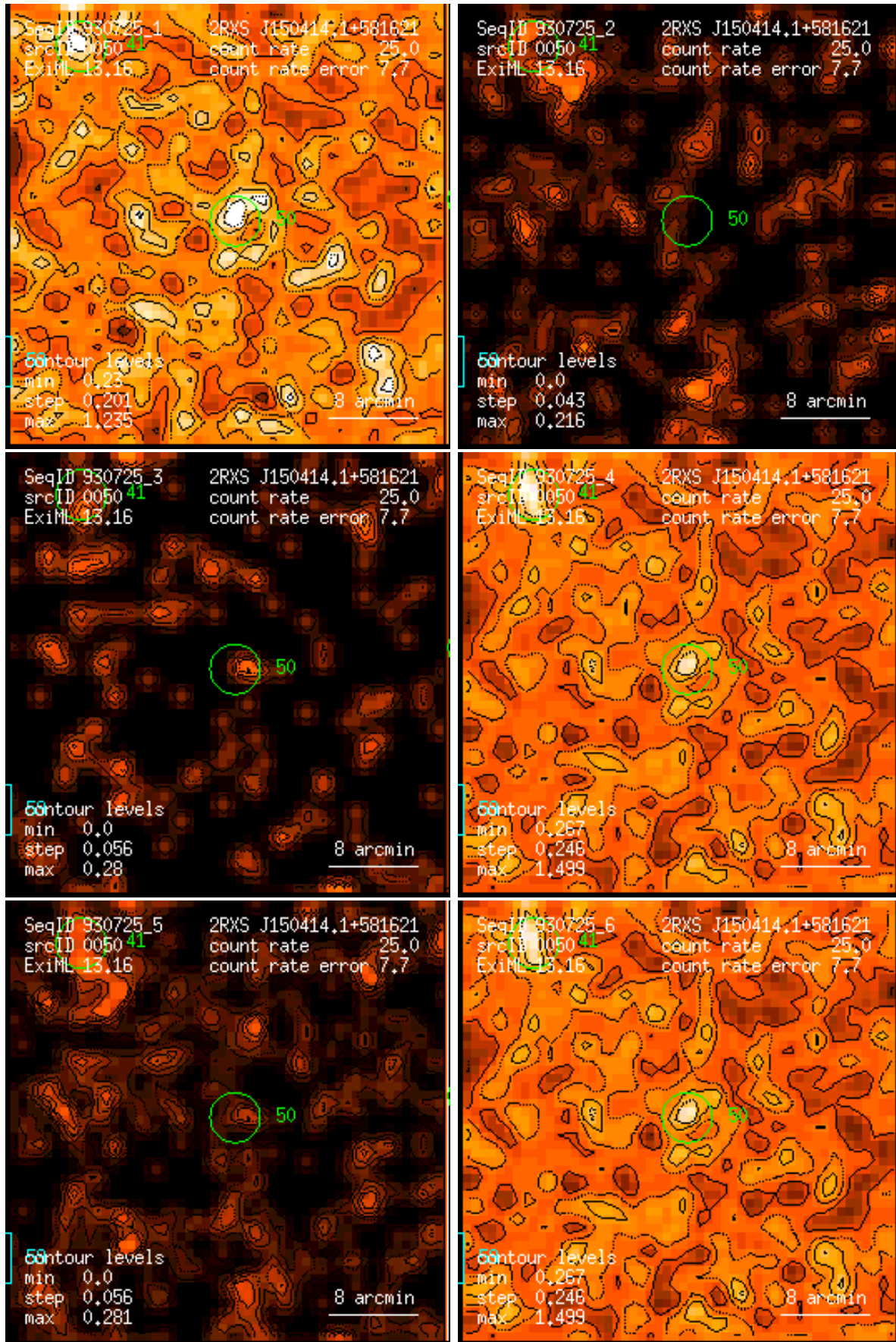
Figure 50: RASS 930725: detection 0050: band rate images, Gaussian filter: (1) PSPC channels 11 – 41, (2) 52 – 90, (3) 91 – 201, (4) 11 – 235, (5) 52 – 201, (6) 11 – 201. Broad band rates in counts/ks. Band rate contour levels in counts/ks/arcmin 2 .
