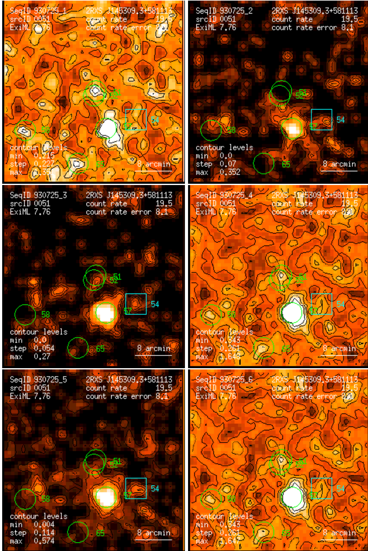
Figure 51: RASS 930725: detection 0051: band rate images, Gaussian filter: (1) PSPC channels 11 – 41, (2) 52 – 90, (3) 91 – 201, (4) 11 – 235, (5) 52 – 201, (6) 11 – 201. Broad band rates in counts/ks. Band rate contour levels in counts/ks/arcmin 2 .
