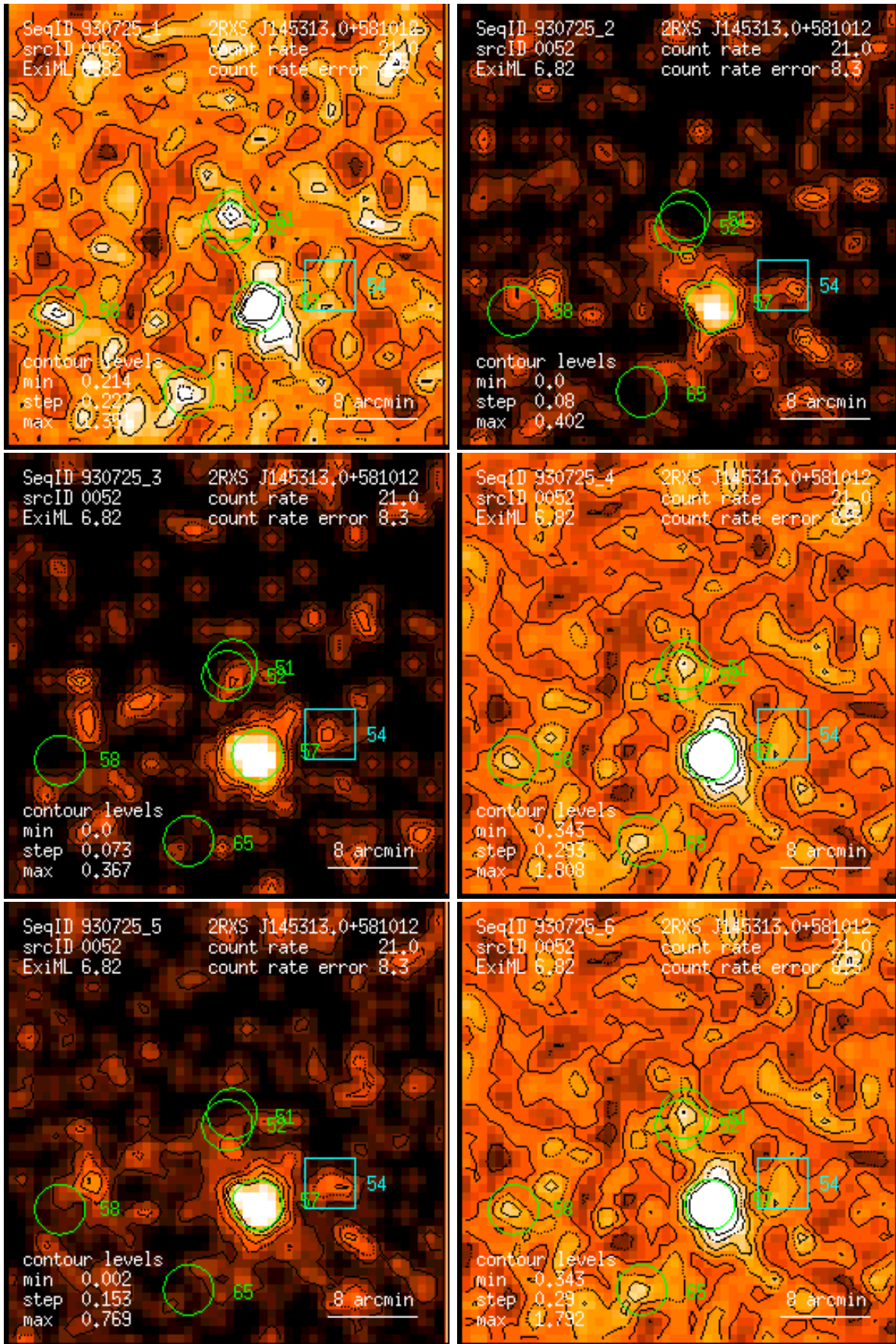
Figure 52: RASS 930725: detection 0052: band rate images, Gaussian filter: (1) PSPC channels 11 – 41, (2) 52 – 90, (3) 91 – 201, (4) 11 – 235, (5) 52 – 201, (6) 11 – 201. Broad band rates in counts/ks. Band rate contour levels in counts/ks/arcmin 2 .
