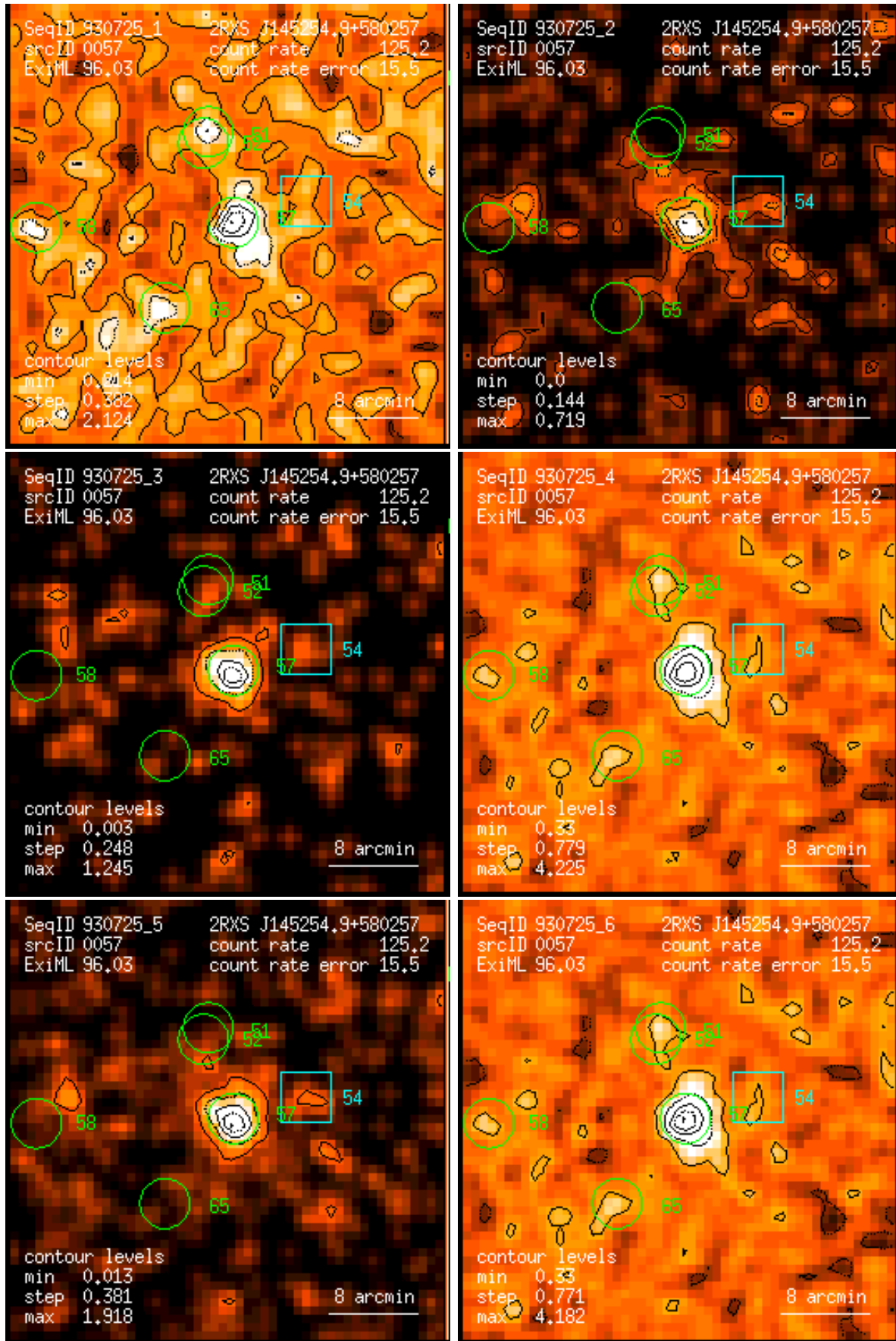
Figure 57: RASS 930725: detection 0057: band rate images, Gaussian filter: (1) PSPC channels 11 – 41, (2) 52 – 90, (3) 91 – 201, (4) 11 – 235, (5) 52 – 201, (6) 11 – 201. Broad band rates in counts/ks. Band rate contour levels in counts/ks/arcmin 2 .
