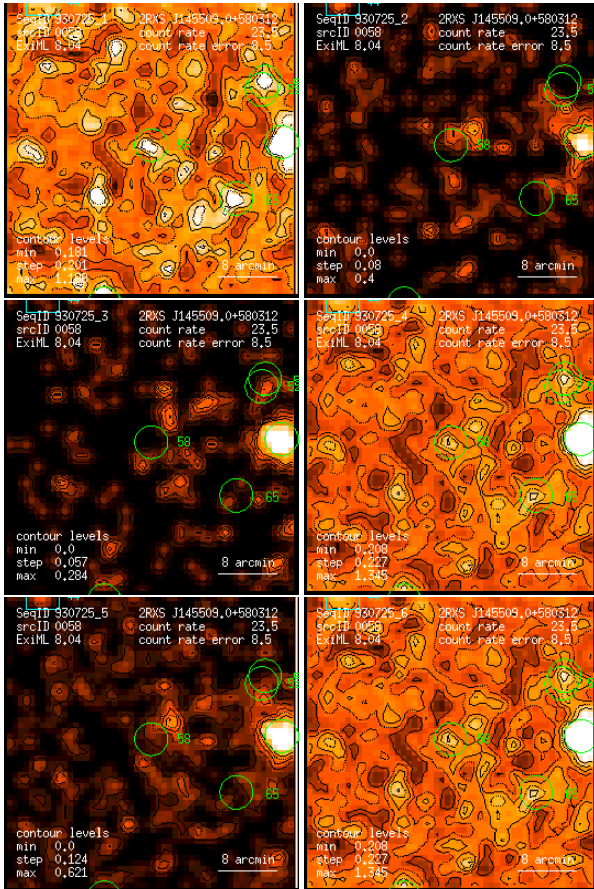
Figure 58: RASS 930725: detection 0058: band rate images, Gaussian filter: (1) PSPC channels 11 – 41, (2) 52 – 90, (3) 91 – 201, (4) 11 – 235, (5) 52 – 201, (6) 11 – 201. Broad band rates in counts/ks. Band rate contour levels in counts/ks/arcmin 2 .
