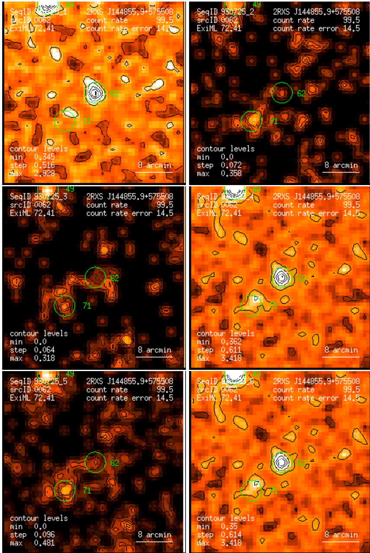
Figure 62: RASS 930725: detection 0062: band rate images, Gaussian filter: (1) PSPC channels 11 – 41, (2) 52 – 90, (3) 91 – 201, (4) 11 – 235, (5) 52 – 201, (6) 11 – 201. Broad band rates in counts/ks. Band rate contour levels in counts/ks/arcmin 2 .
