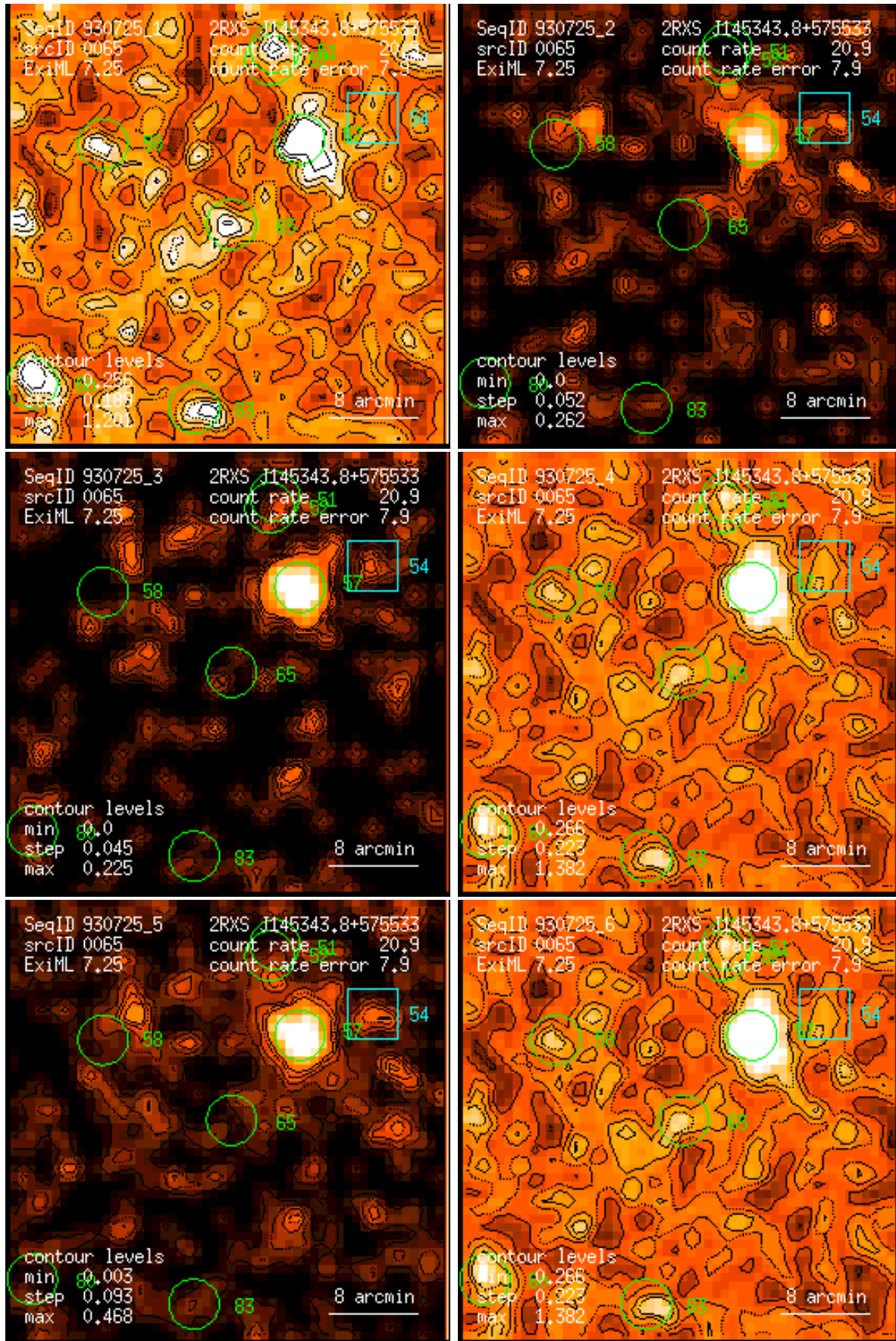
Figure 65: RASS 930725: detection 0065: band rate images, Gaussian filter: (1) PSPC channels 11 – 41, (2) 52 – 90, (3) 91 – 201, (4) 11 – 235, (5) 52 – 201, (6) 11 – 201. Broad band rates in counts/ks. Band rate contour levels in counts/ks/arcmin 2 .
